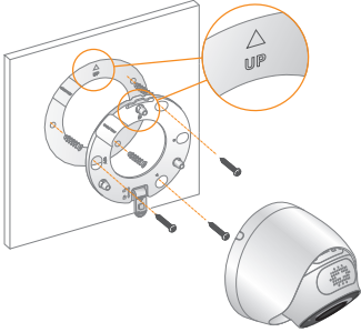
Figure 4-2 Wall mount
