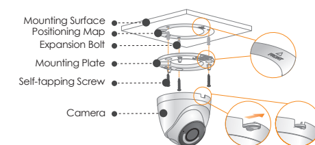
Figure 4-1 Installation diagram
