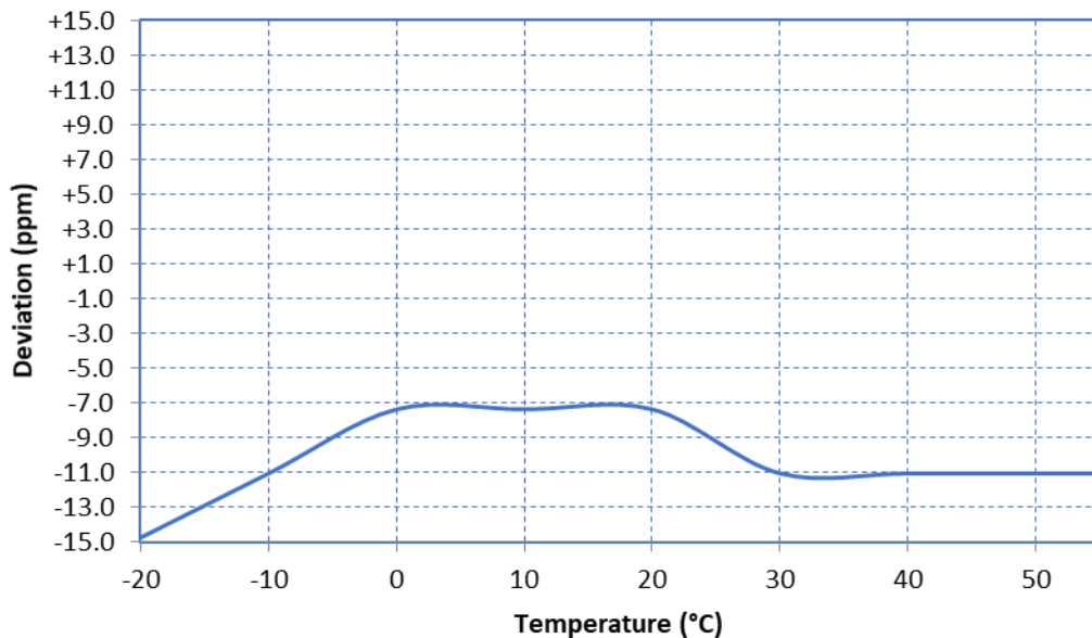
Frequency Stability
