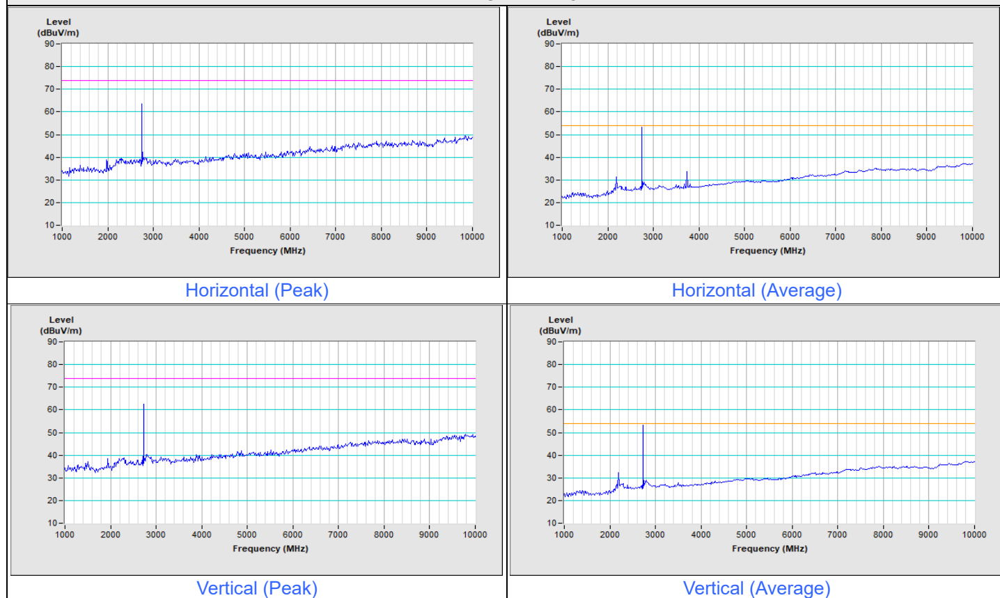
RFID Channel 25
