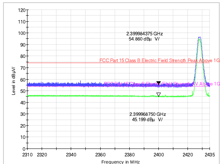
Electric Field Strength 1-18GdBuV TX Band Edge+EIRP
