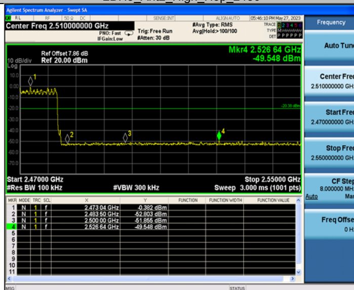
2DH5_Ant2_High_Hop_2480
