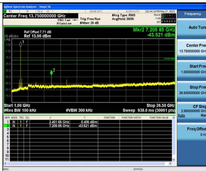
DH5_Ant2_2402_0~Reference
