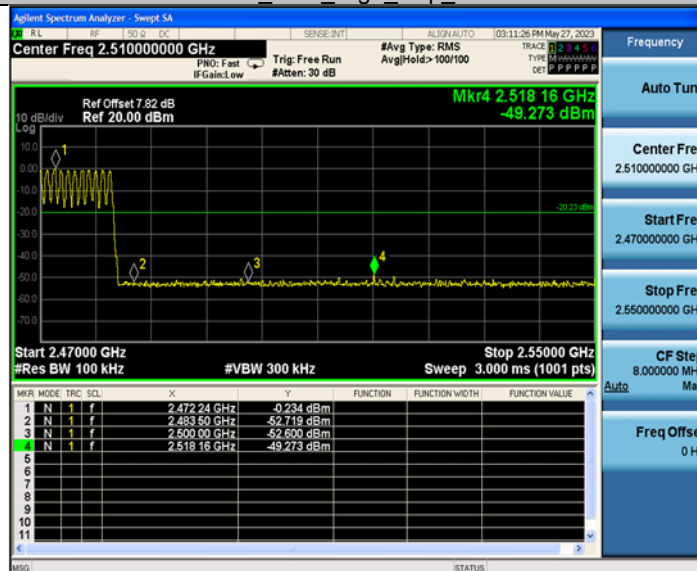
DH5_Ant2_High_Hop_2480
