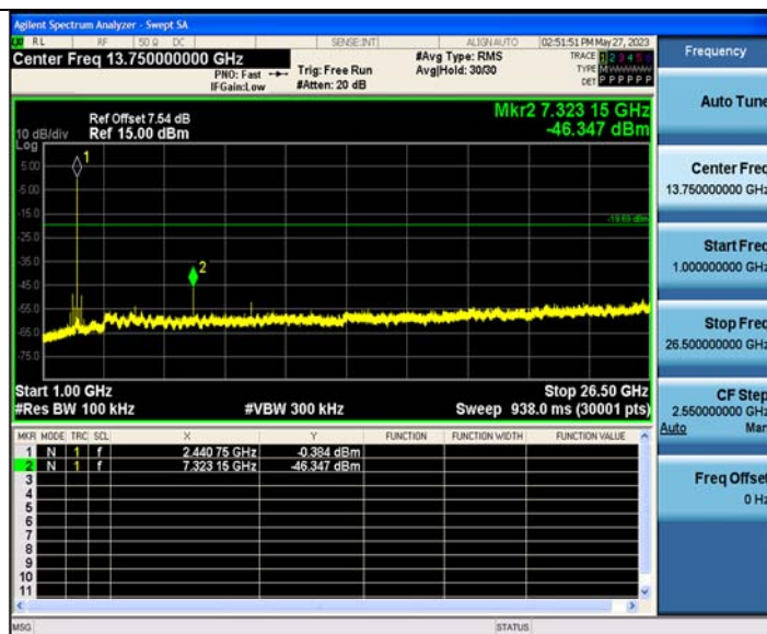
DH5_Ant2_2441_0~Reference
