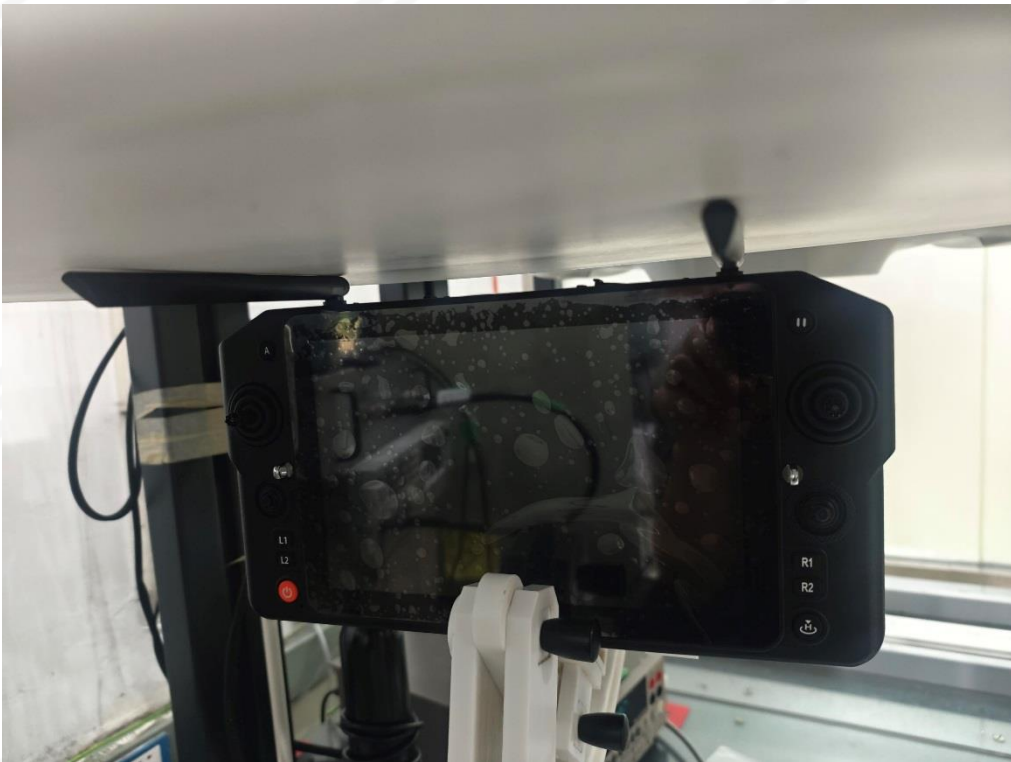
Body Top Side Antenna Horizontal (separation distance is 0mm)
