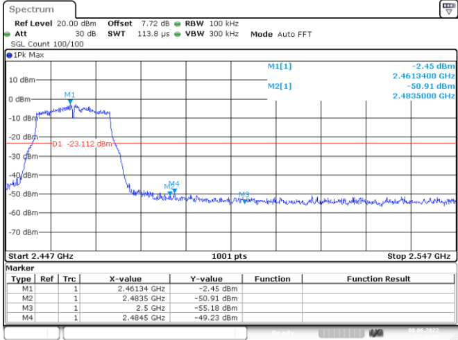
Band Edge NVNT g 2462MHz Ant1 Emission
