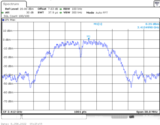
Band Edge NVNT b 2412MHz Ant1 Emission
