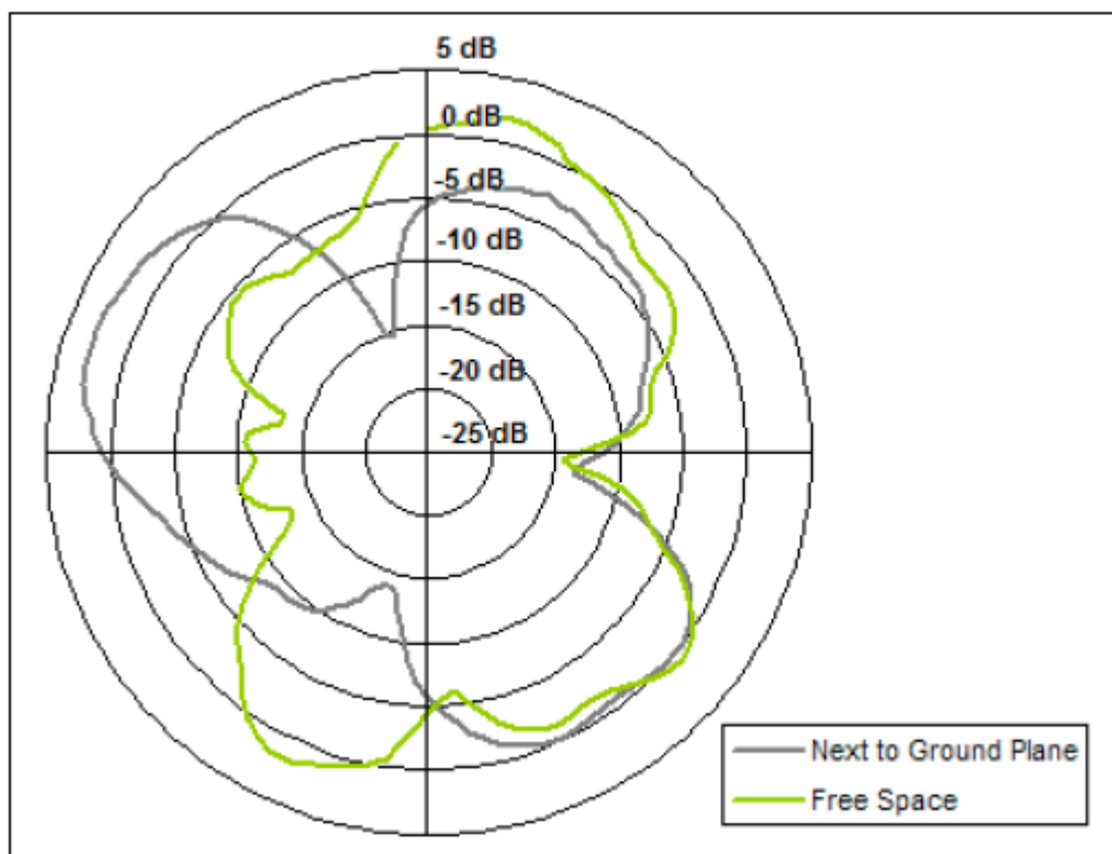
Figure 10. Radiation pattern data YZ for Antenna
