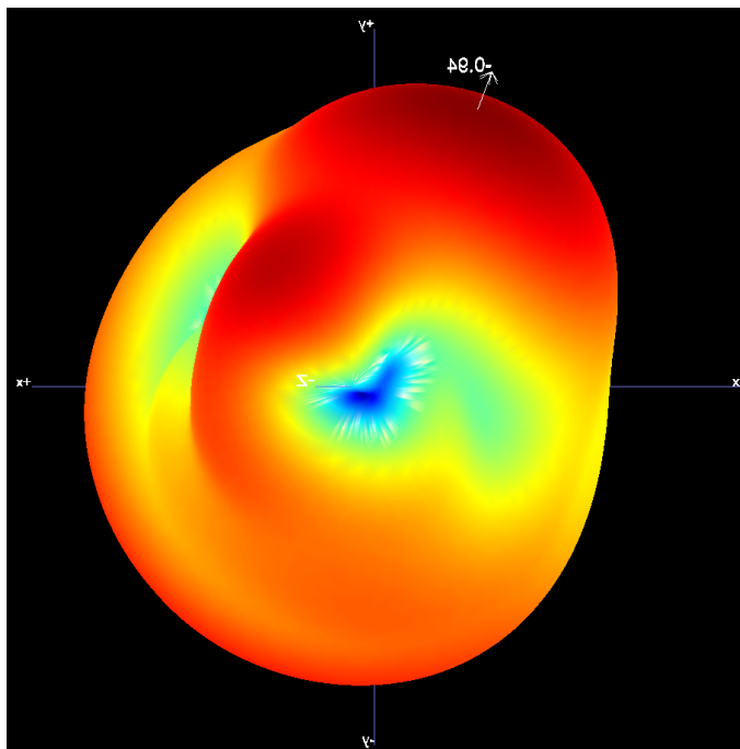
B1.2 3D Pattern for 2450MHz
