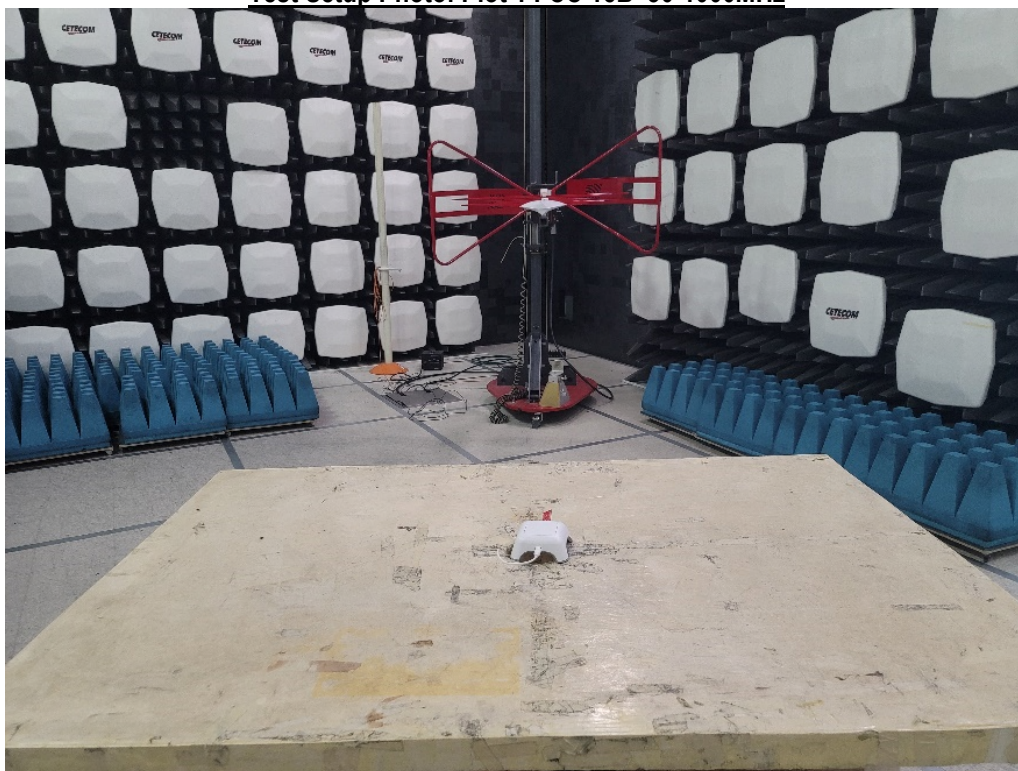
Test Setup Photo: Plot 1 FCC 15B 30-1000MHz
