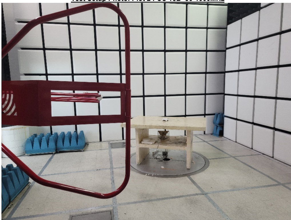
Test Setup Photo: Plot 2 FCC 15B 30-1000MHz
