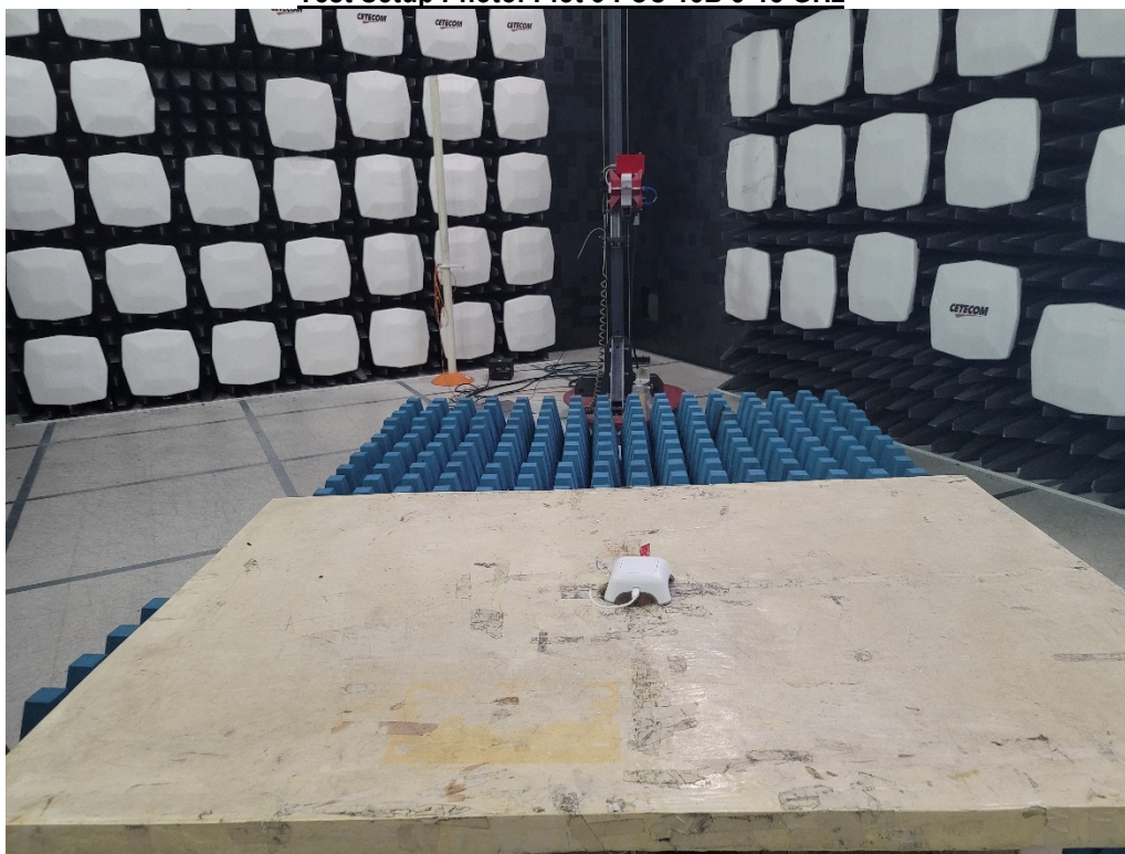
Test Setup Photo: Plot 3 FCC 15B 3-18 GHz
