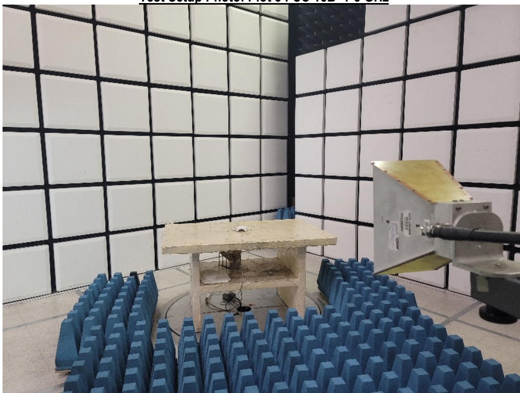
Test Setup Photo: Plot 3 FCC 15B 1-3 GHz
