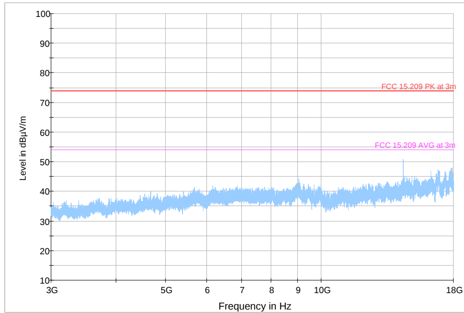
Plot # 18. Radiated Emissions: 3-18 GHz
