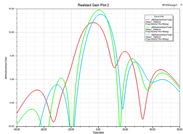
Elevation/Vertical
