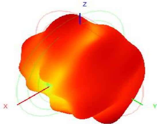
2450.0MHz H+V, Eff: 7.0%
