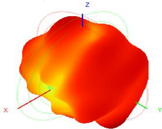
2440.0MHz H+V, Eff: 6.7%
