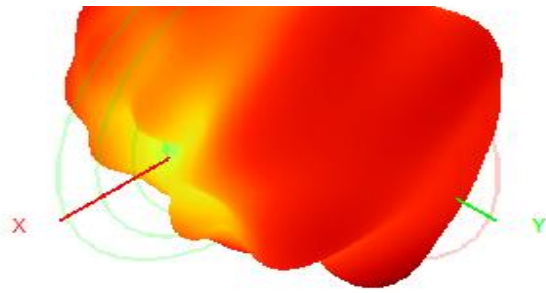
2440.0MHz H+V, Eff: 6.7%
