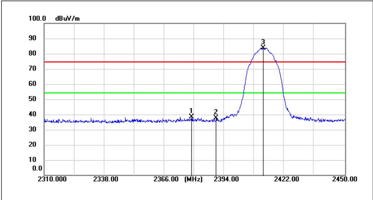
11b_TX_CH_01_Vertical_Peak
