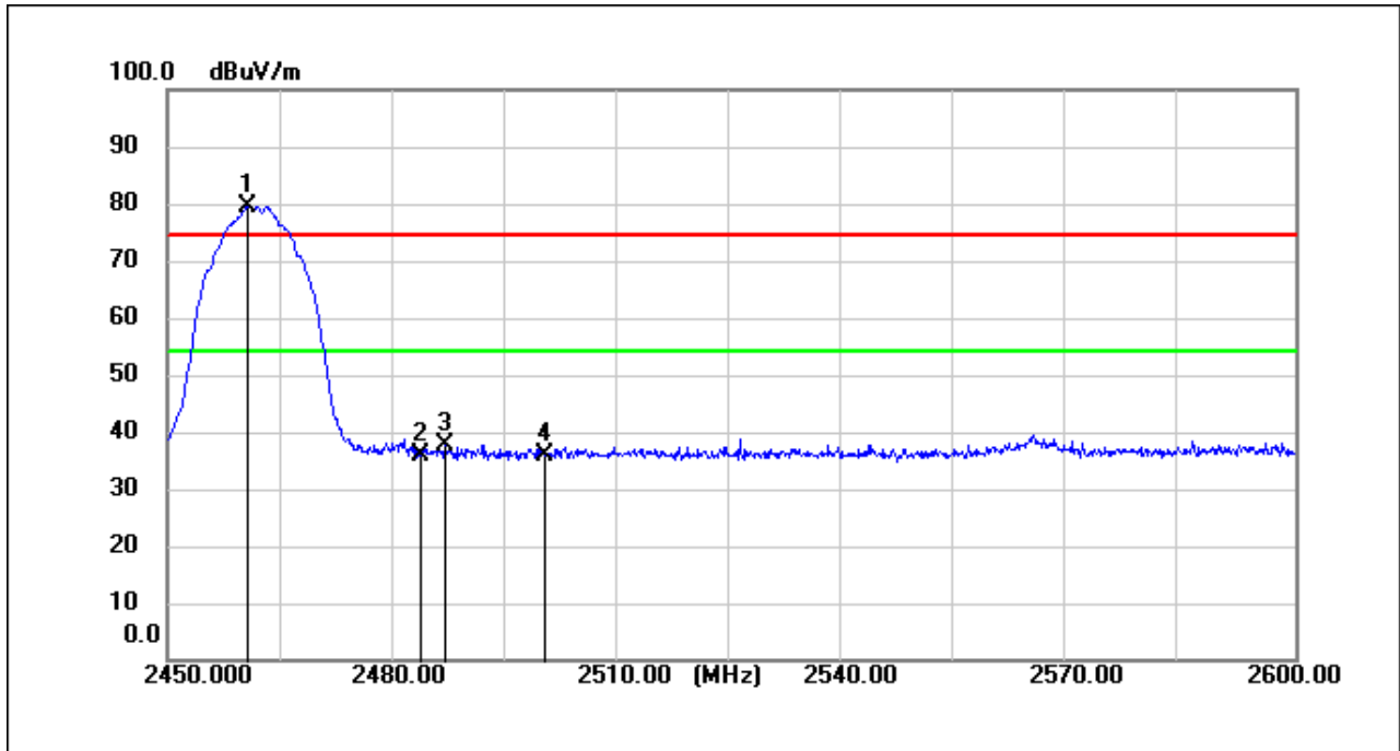
11b_TX_CH_11_Vertical_Peak
