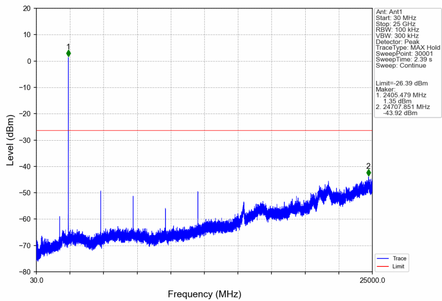
Zigbee_LCH_2405MHz_Ant1_NTNV
