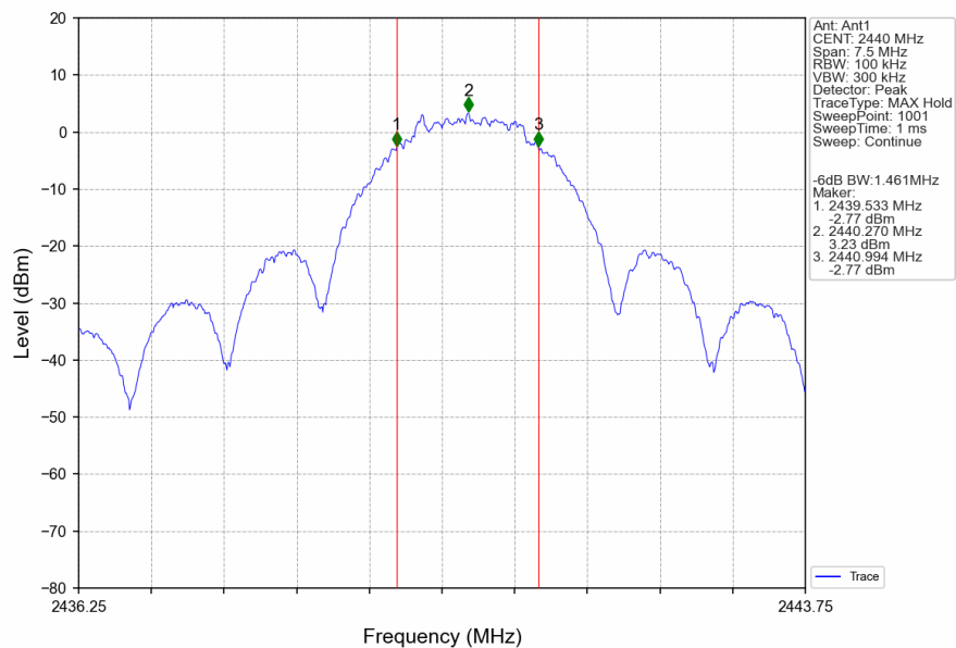
Zigbee_MCH_2440MHz_Ant1_NTNV
