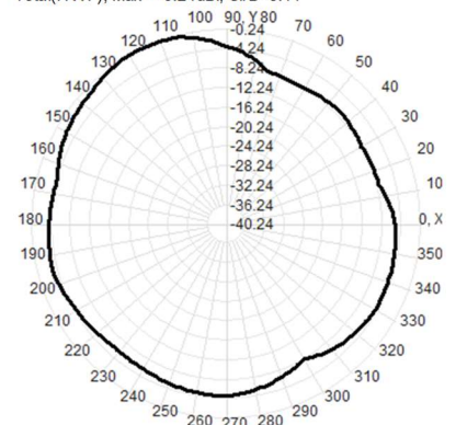
Total(H-XY), Max= -0.24dBi, CirD=8.11
