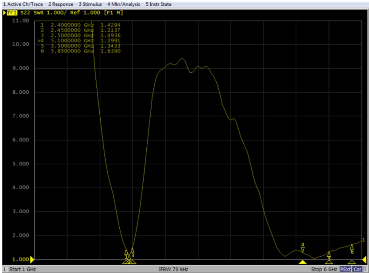
K 3D&K6D antenna VSWR
