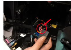
11. Plug the fiber cable to CarPlay box 48PIN connector
