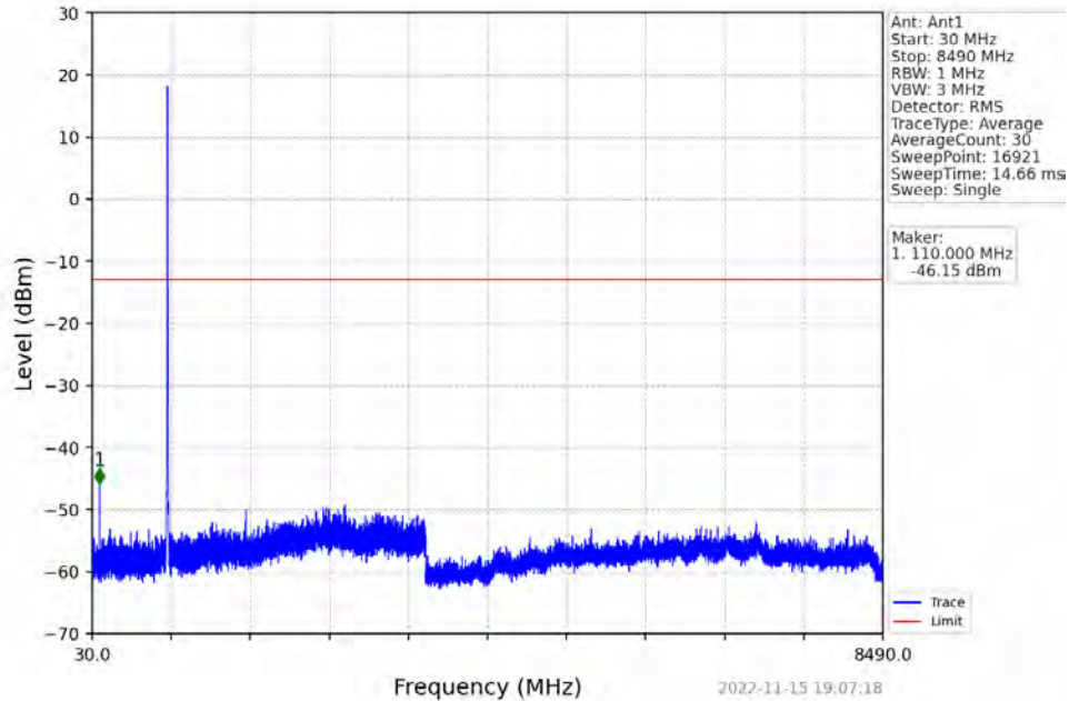
Band5_RMC_HCH_846.6MHz_12.2kbps RMC_NTNV
