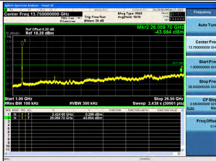
11N40SISO_Ant1_2437_0~Reference
