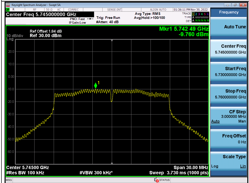
Test_Graph_802.11n20_ANT2_5745_MCS0_PSD
