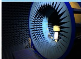
SATIMO-16
