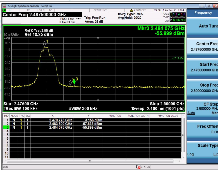
2_Bandedge_NVNT_ANT1_1Mbps_2480
