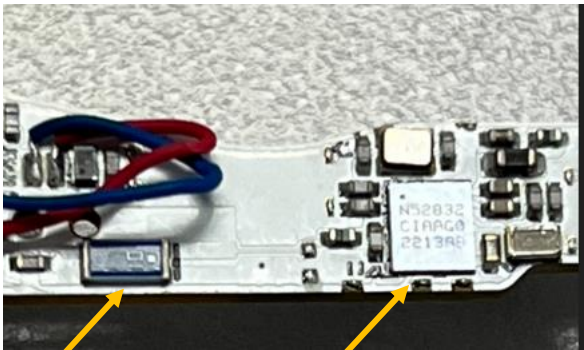
Chip Antenna
