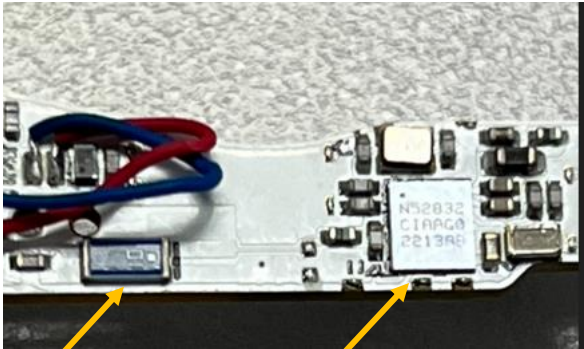
Chip Antenna
