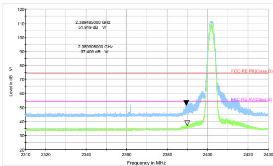
Bluetooth LE (2M) Channel 0 Peak &amp; Average
