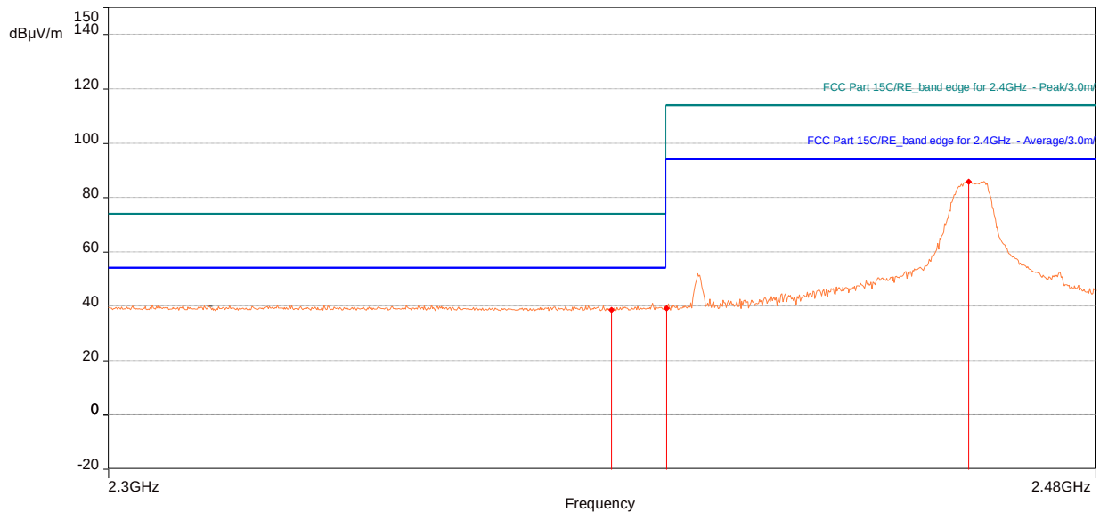
2456MHz Vertical
