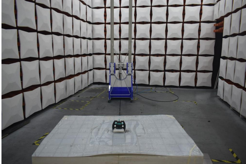
TX 30MHz~1GHz
