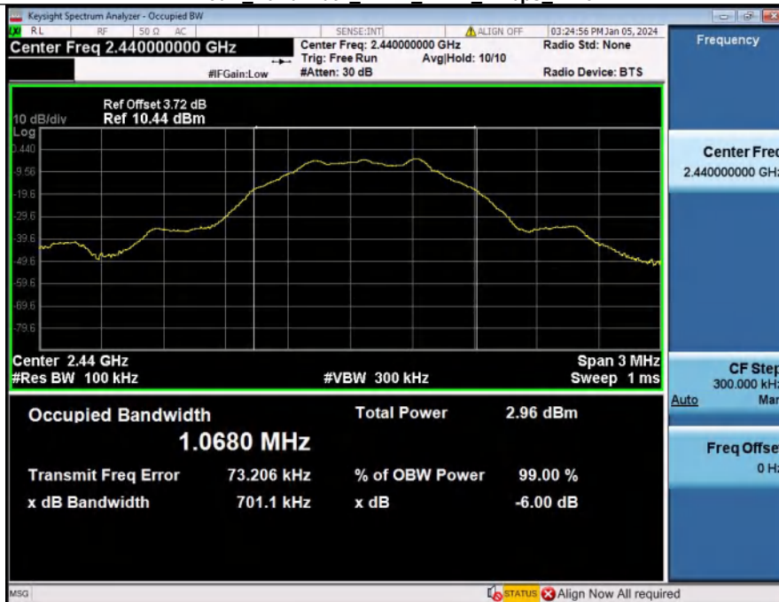
-6dB Bandwidth_NVNT_ANT1_1Mbps_2440
