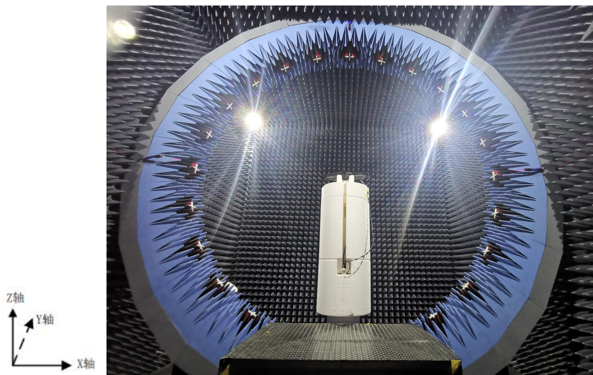
Front view
