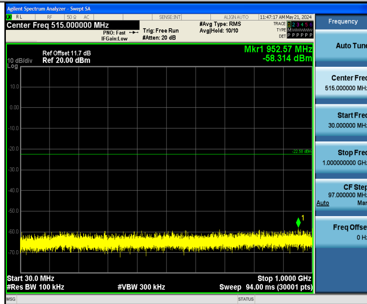
3DH5-Ant1-2480-30~1000-PASS
