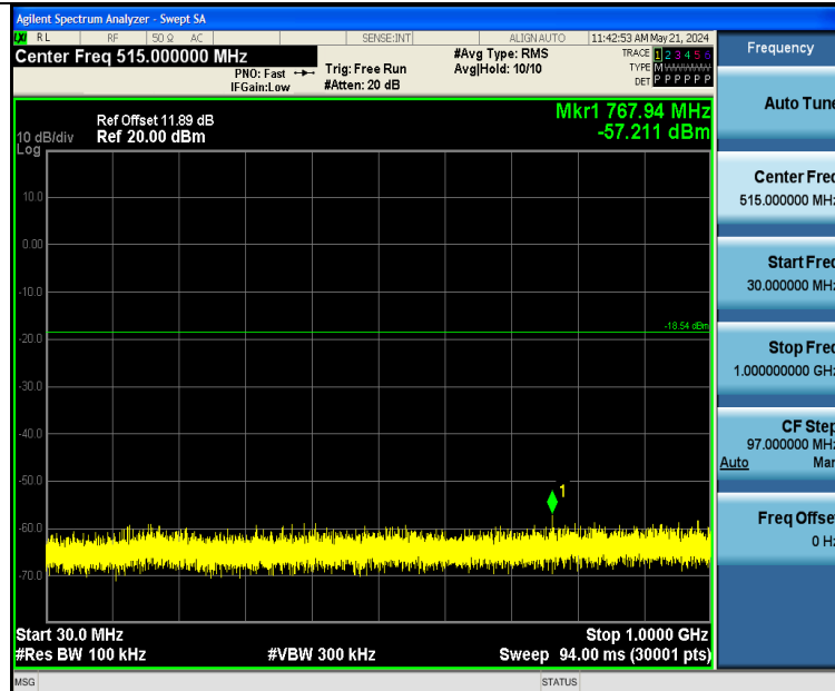
3DH5-Ant1-2402-30~1000-PASS
