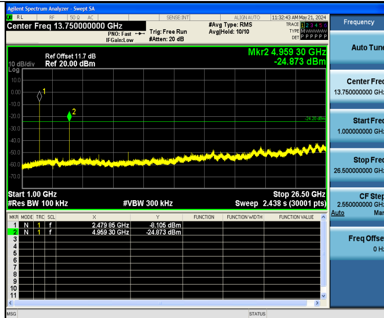
2DH5-Ant1-2480-1000~26500-PASS
