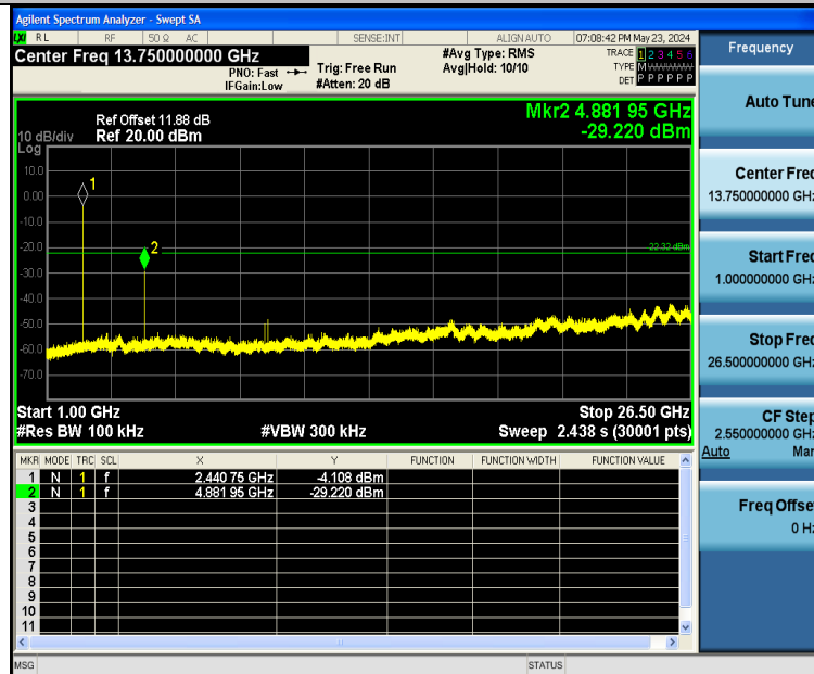
2DH5-Ant1-2441-1000~26500-PASS
