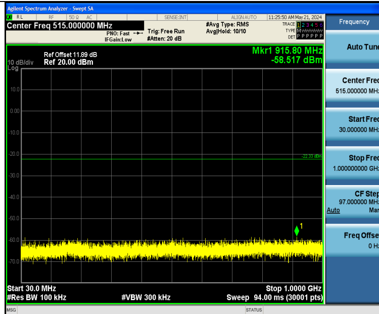
2DH5-Ant1-2402-30~1000-PASS
