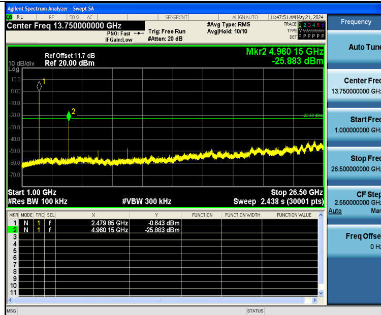
3DH5-Ant1-2480-1000~26500-PASS
