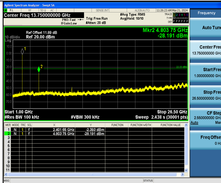
2DH5-Ant1-2402-1000~26500-PASS
