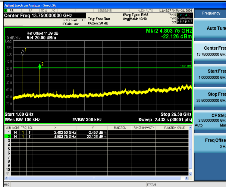
3DH5-Ant1-2402-1000~26500-PASS
