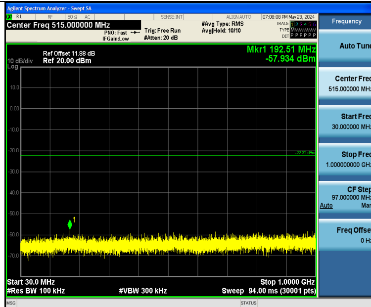
2DH5-Ant1-2441-30~1000-PASS
