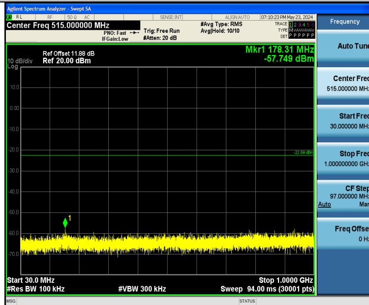
3DH5-Ant1-2441-30~1000-PASS
