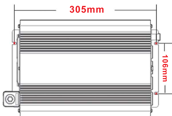
4000 Watts
