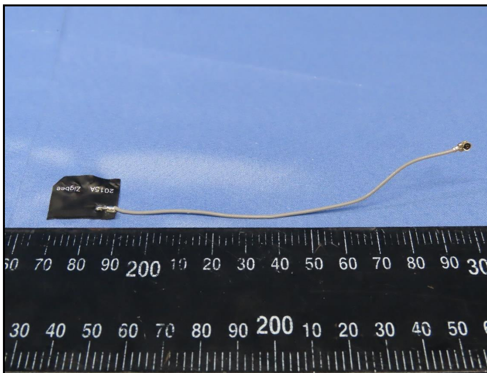
Antenna No.2 (802.15.4)
