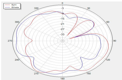
H Theta=90 freq=2440MHz
