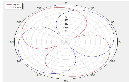
H Theta=0 freq=2440MHz
