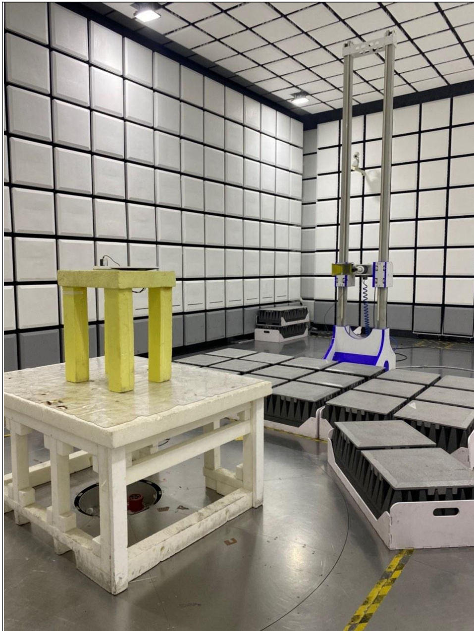
RADIATED EMISSION TEST (Above 1GHz) Part 15C
