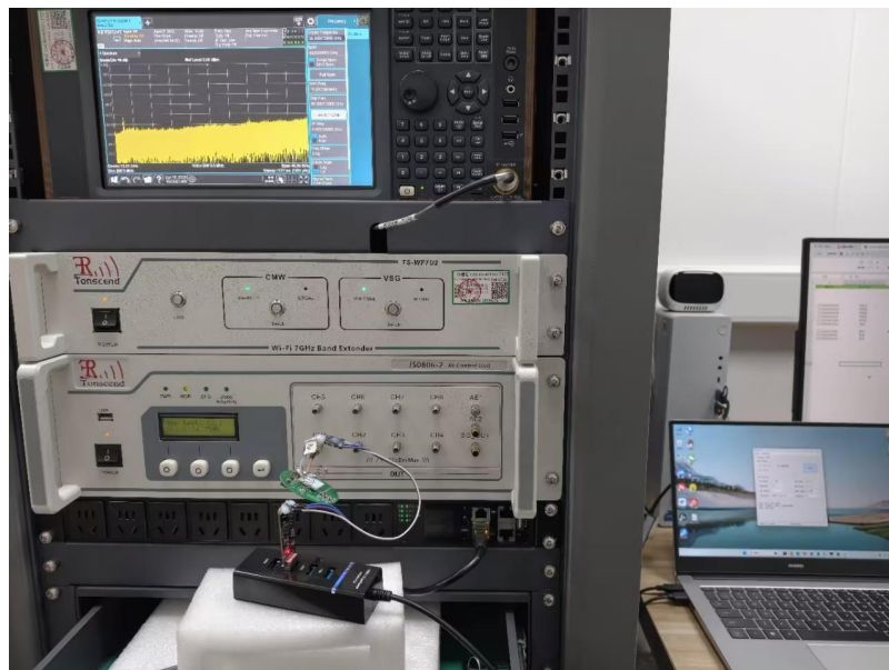
RF conducted
