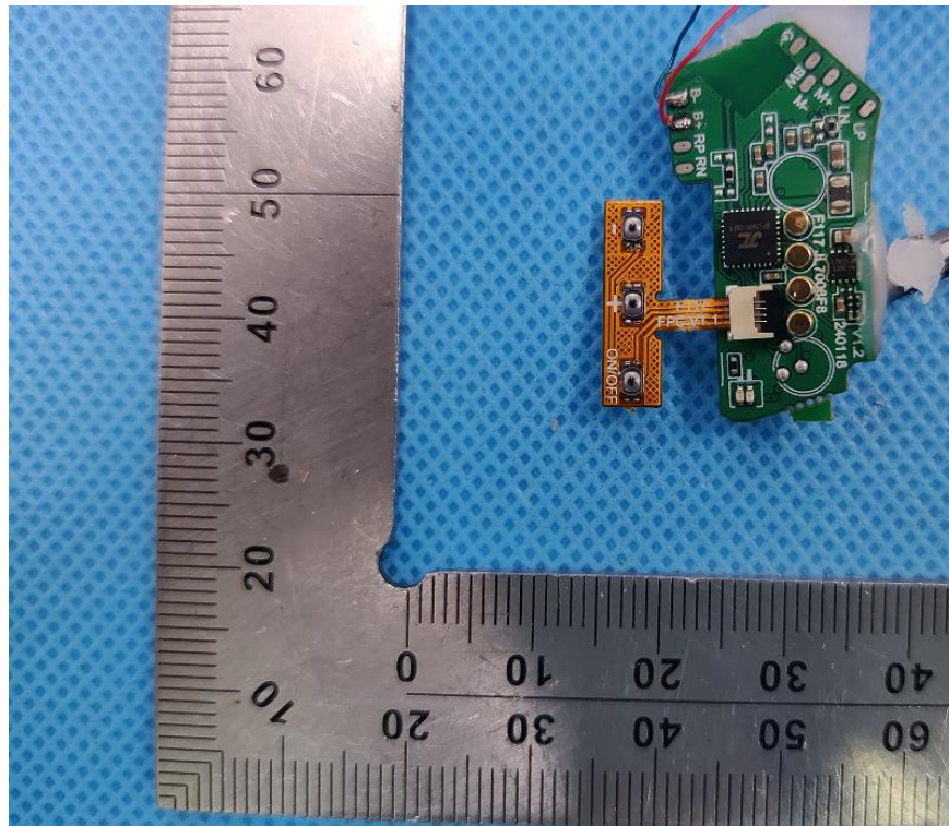
INTERNAL VIEW OF EUT (FIGURE 3)
