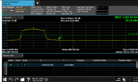
Out Of Band Emission IEEE 802.11n_Channel 11_20MHz_Antenna 0
