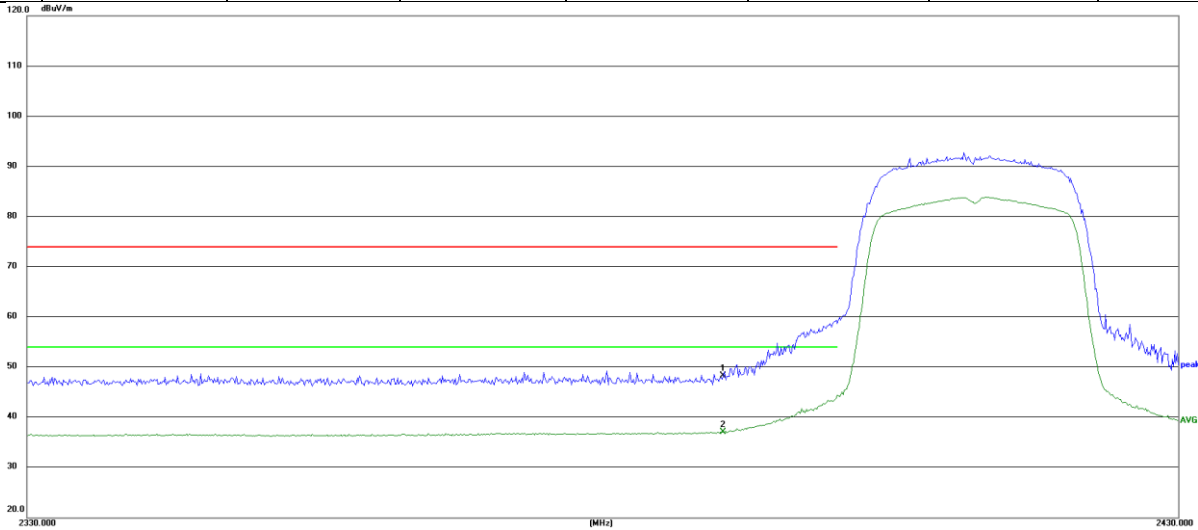
Low Channel (2412 MHz)(802.11n20)—Horizontal
