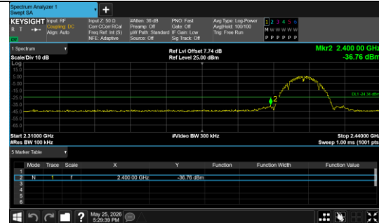
Out Of Band Emission IEEE 802.11b_Channel 1_20MHz_Antenna 0
