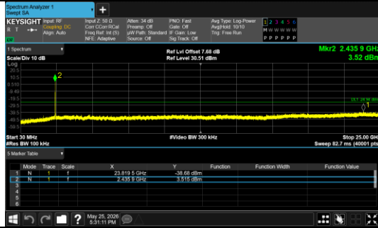
30.0 MHz - 25000.0 MHz IEEE 802.11b_Channel 6_20MHz_Antenna 0
