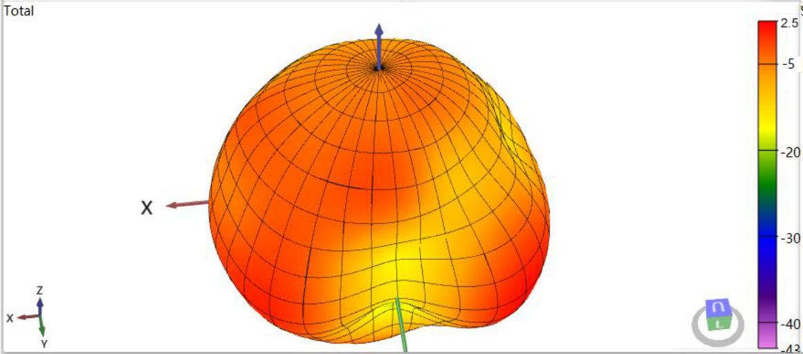
2480MHz 3D-Total Pattern
