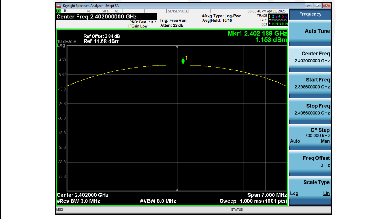
Peak_Output_Power_NVNT_ANT1_2-DH1_2402_00
