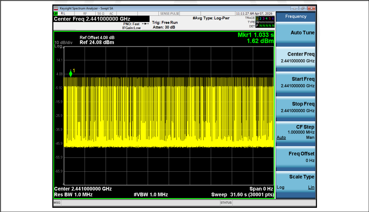
Dwell_Time_(Hopping)_NVNT_ANT1_3-DH1_2441_00_Accumulated
