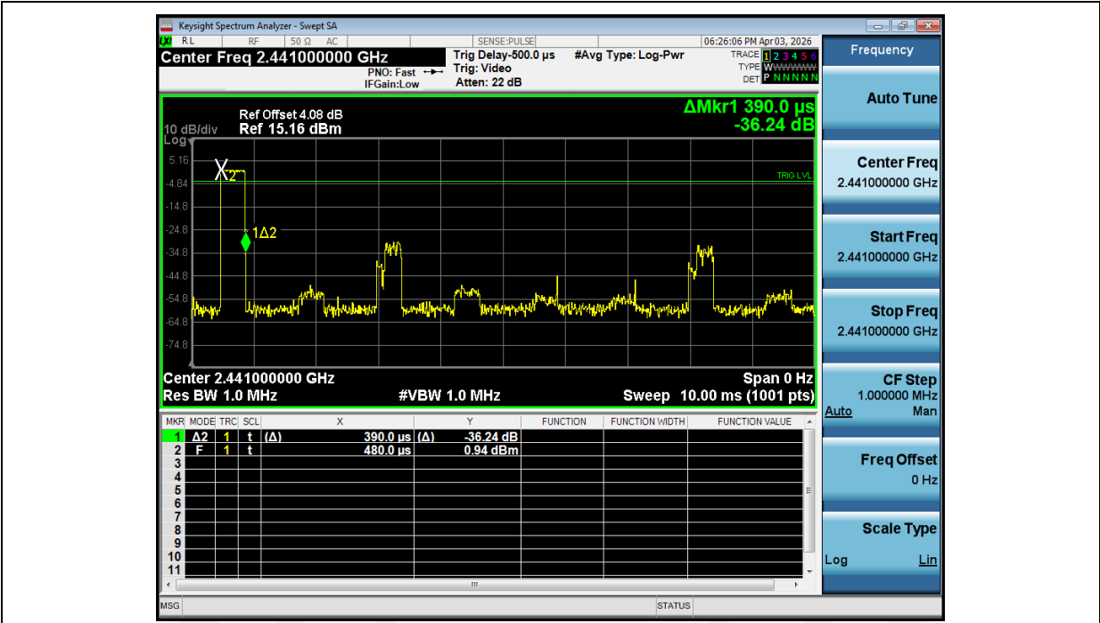
Dwell_Time_(Hopping)_NVNT_ANT1_2-DH1_2441_00_Accumulated
