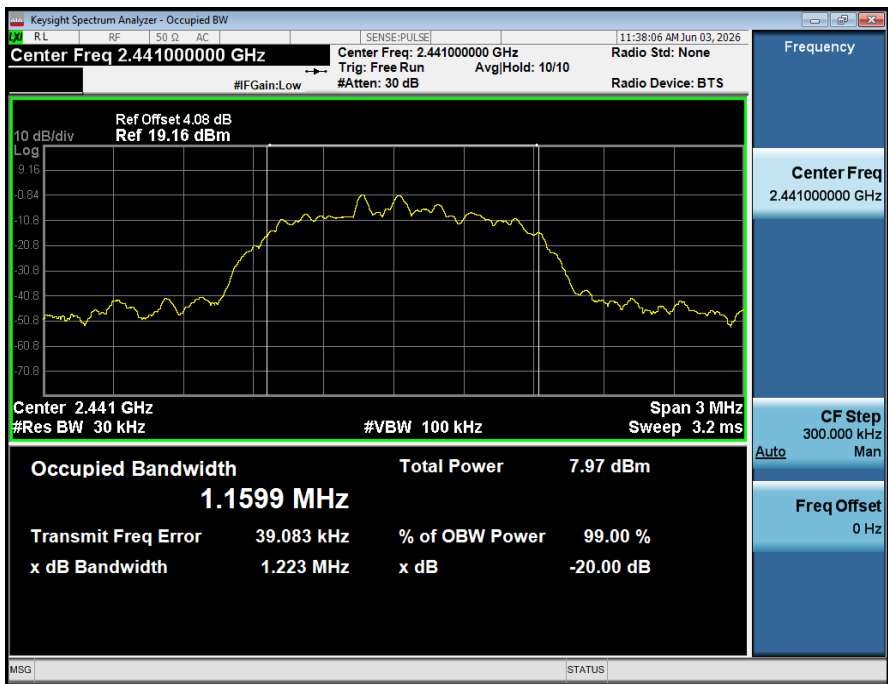
-20dB_Bandwidth_NVNT_ANT1_3-DH1_2441_00
