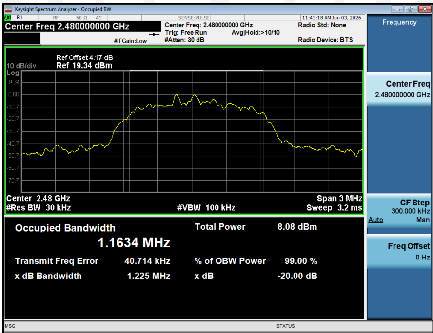
-20dB_Bandwidth_NVNT_ANT1_3-DH1_2480_00
