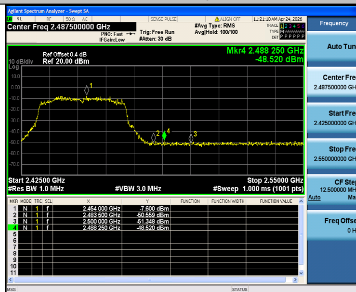
11AX40SISO_Ant2_High_2452_Peak
