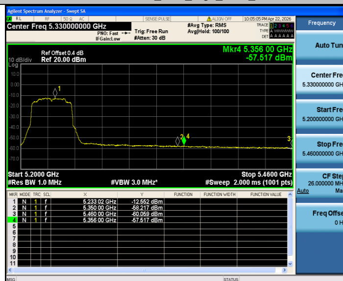
11AX40SISO_Ant2_High_5230_AV
