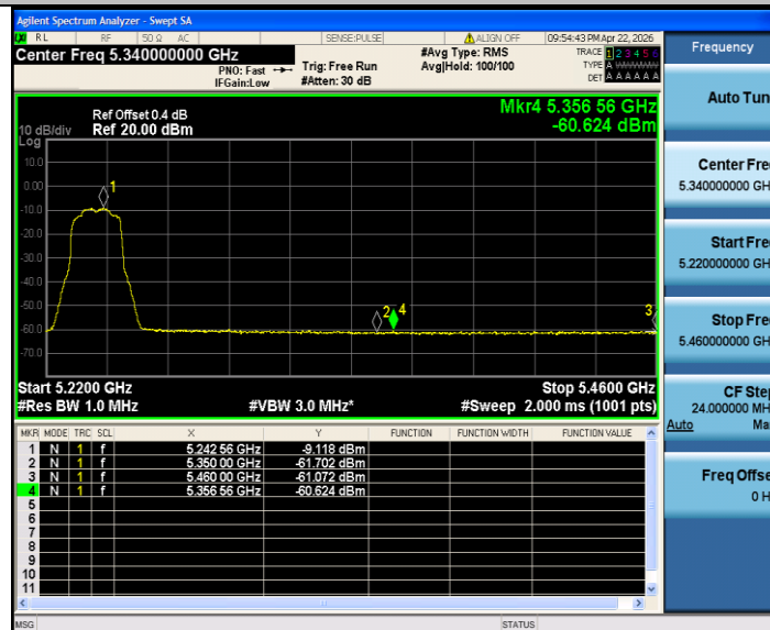
11AX20SISO_Ant2_High_5240_Peak
