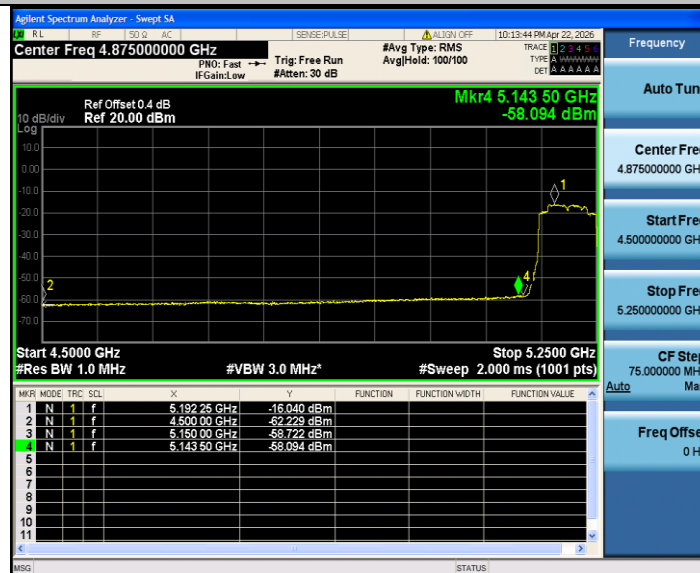
11AX80SISO_Ant2_Low_5210_Peak
