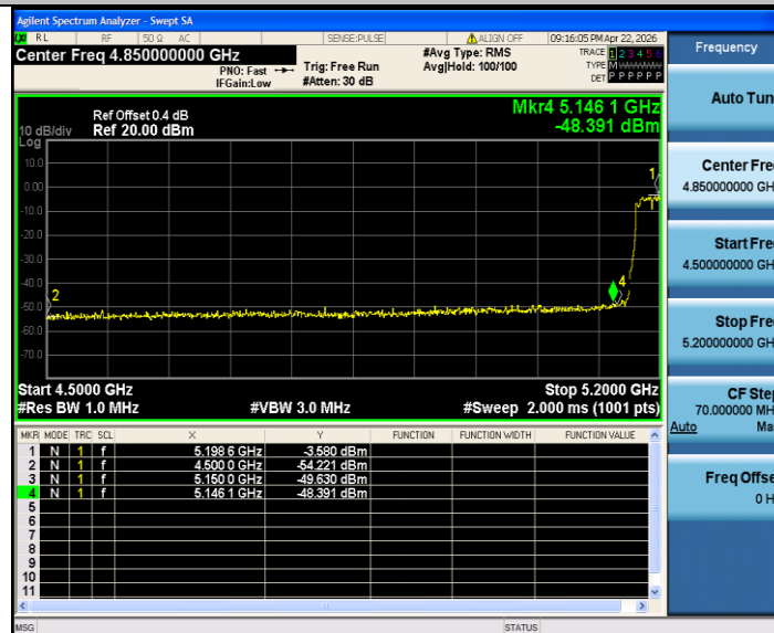
11N40SISO_Ant2_High_5230_AV
