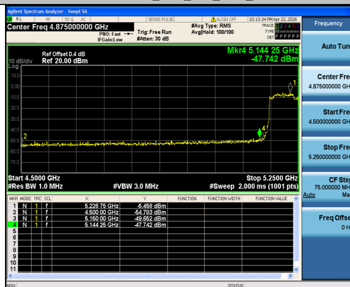
11AX80SISO_Ant2_Low_5210_Peak
