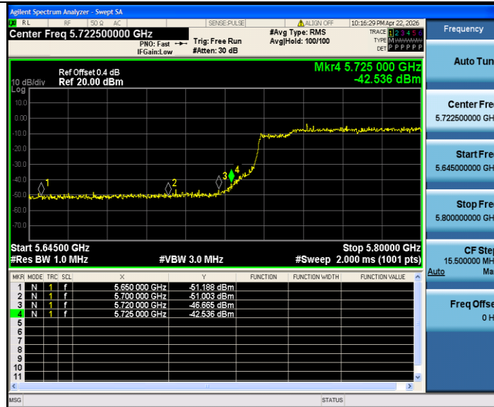
11AX80SISO_Ant2_High_5775_Peak
