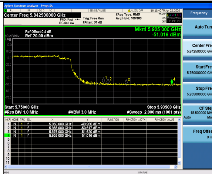
11AX80SISO_Ant2_High_5775_Peak
