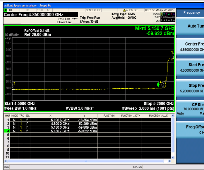
11AX40SISO_Ant1_Low_5190_Peak
