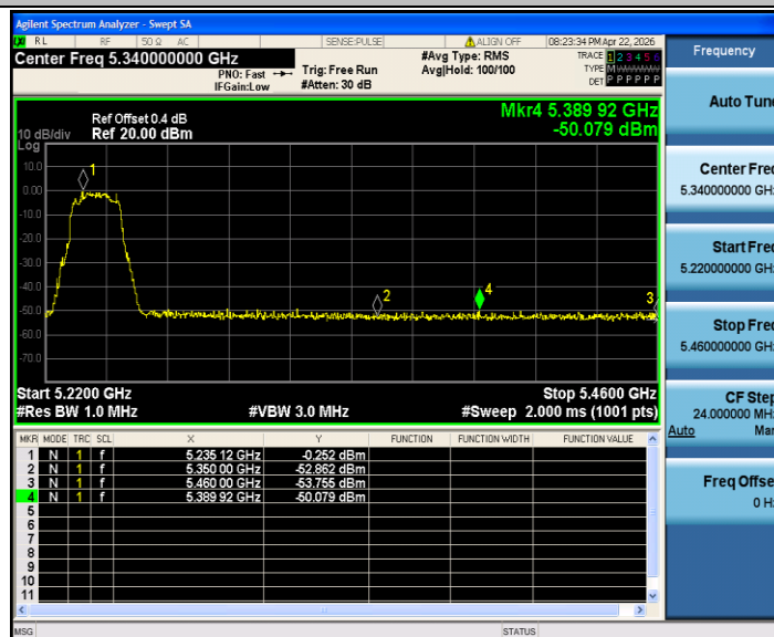
11AX20SISO_Ant1_High_5240_Peak
