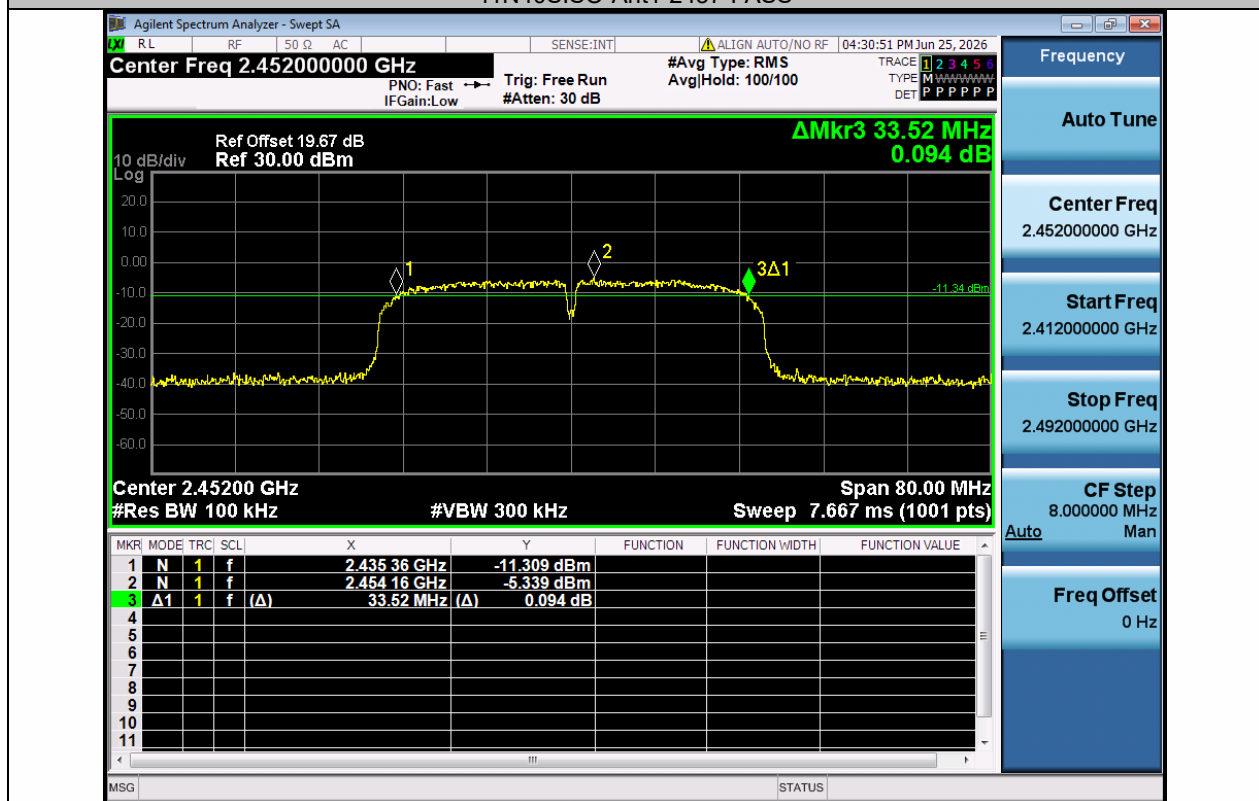
11N40SISO-Ant1-2452-PASS
