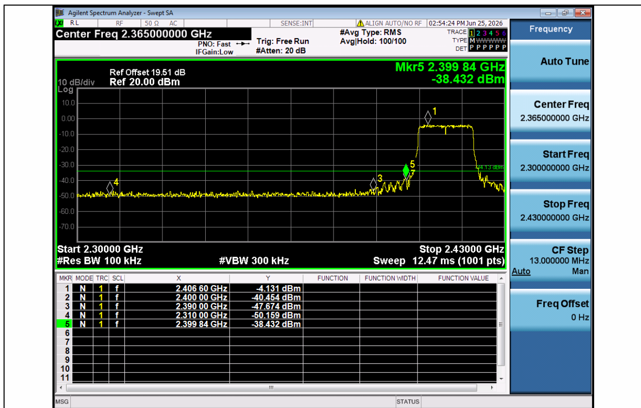
11G-Ant1-2412-PASS
