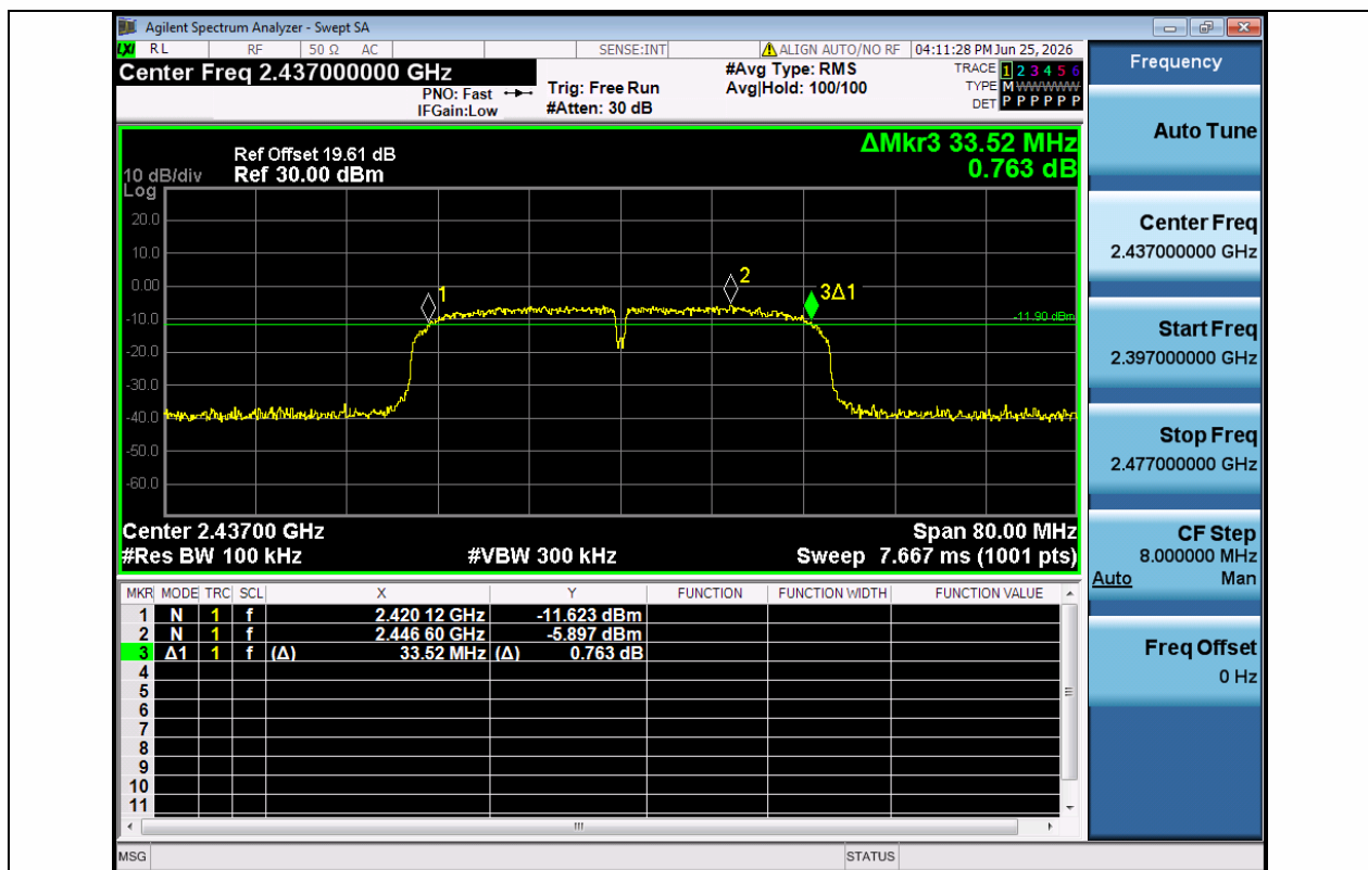
11N40SISO-Ant1-2437-PASS
