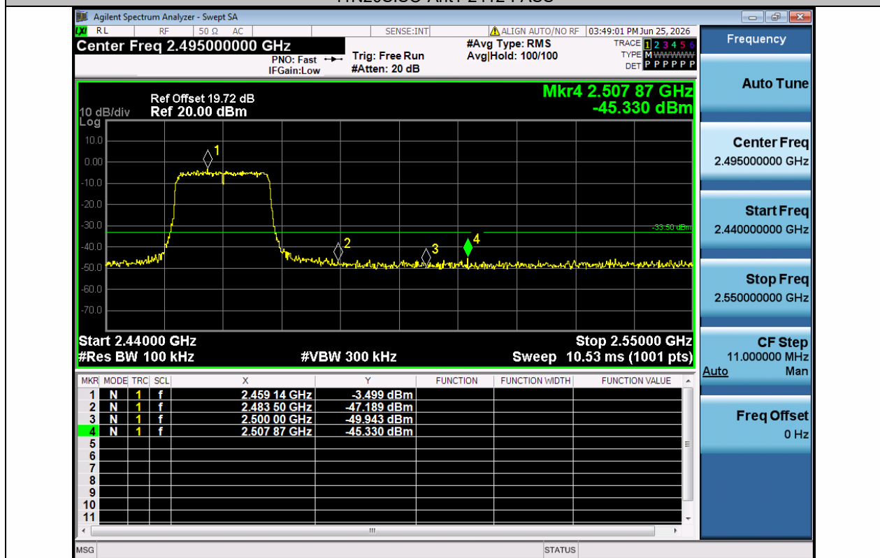
11N20SISO-Ant1-2462-PASS
