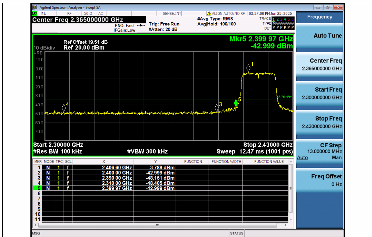
11N20SISO-Ant1-2412-PASS
