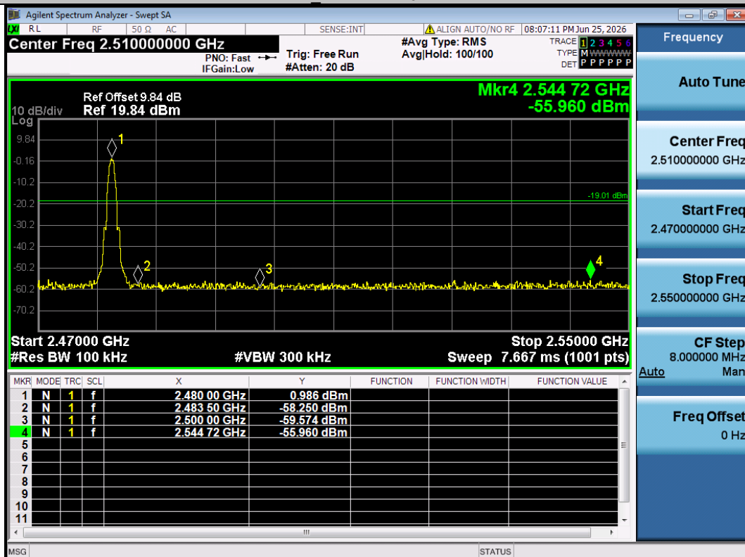
BLE_1M-Ant1-2480-PASS
