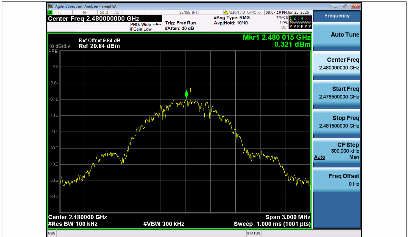
BLE_1M-Ant1-2480-0~Reference-PASS
