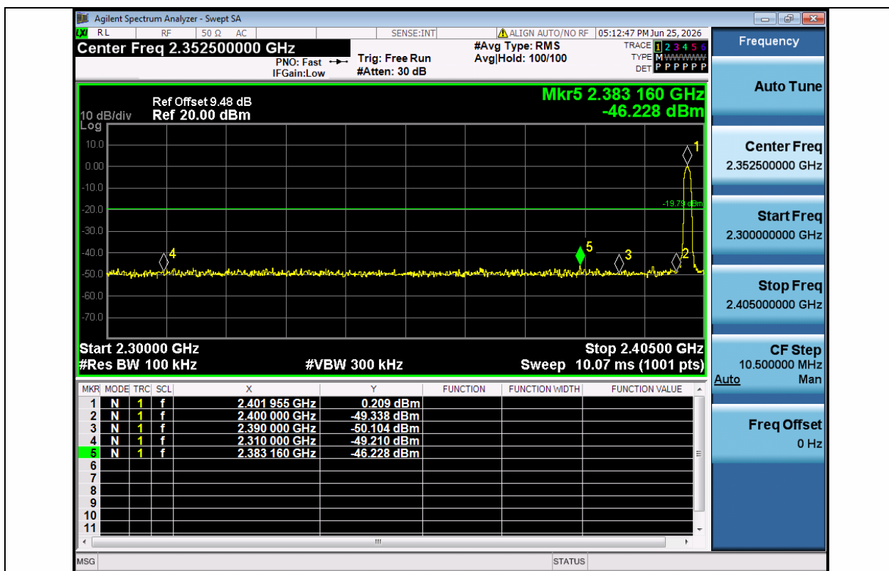
2DH5-Ant1-2402-PASS
