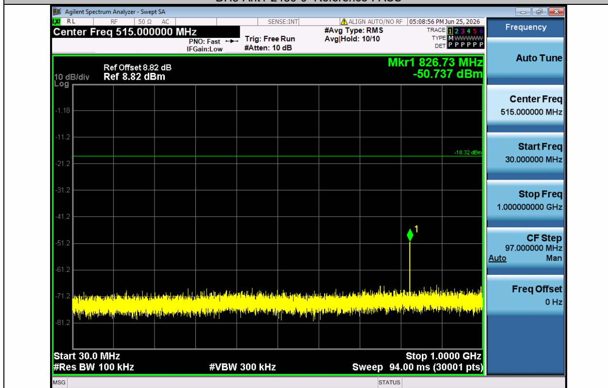
DH5-Ant1-2480-30~1000-PASS
