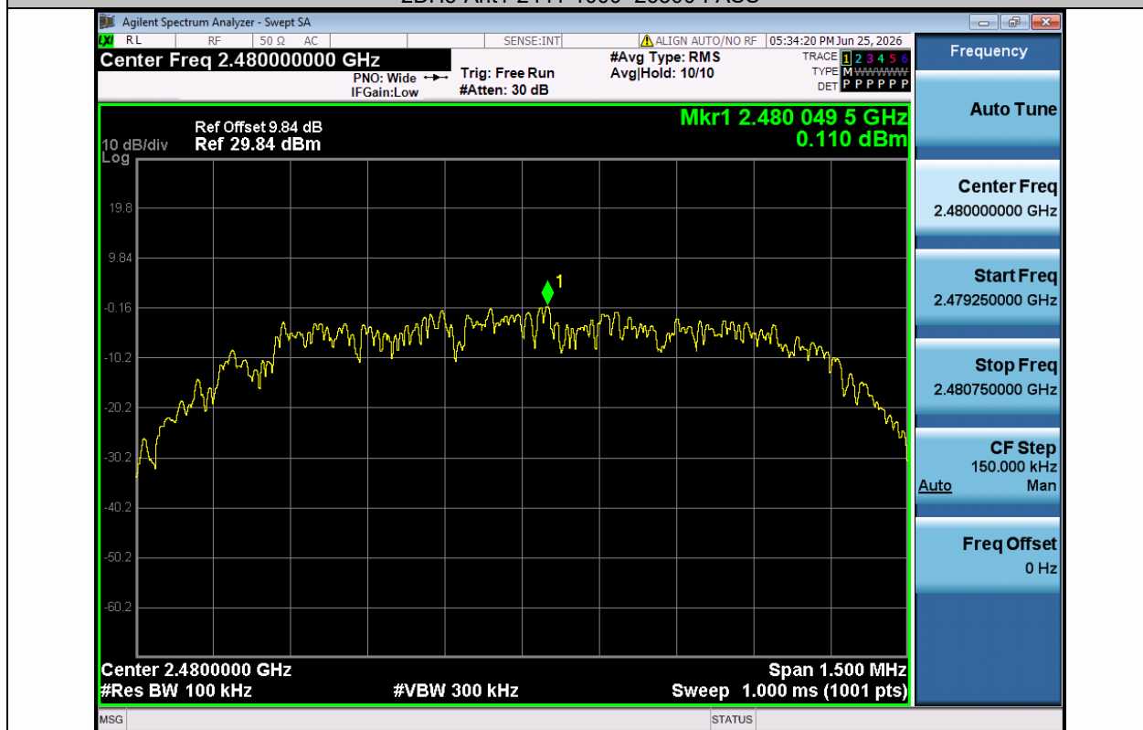
2DH5-Ant1-2480-0~Reference-PASS
