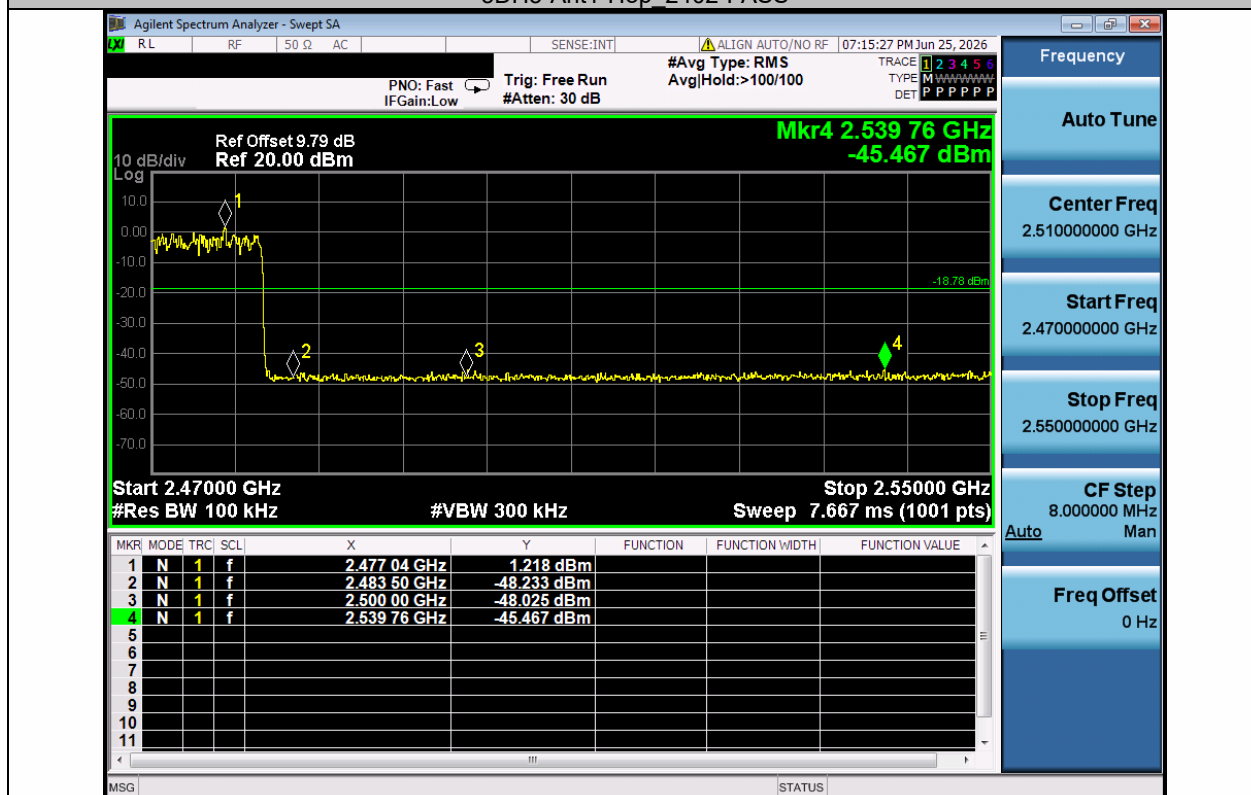
3DH5-Ant1-Hop_2480-PASS
