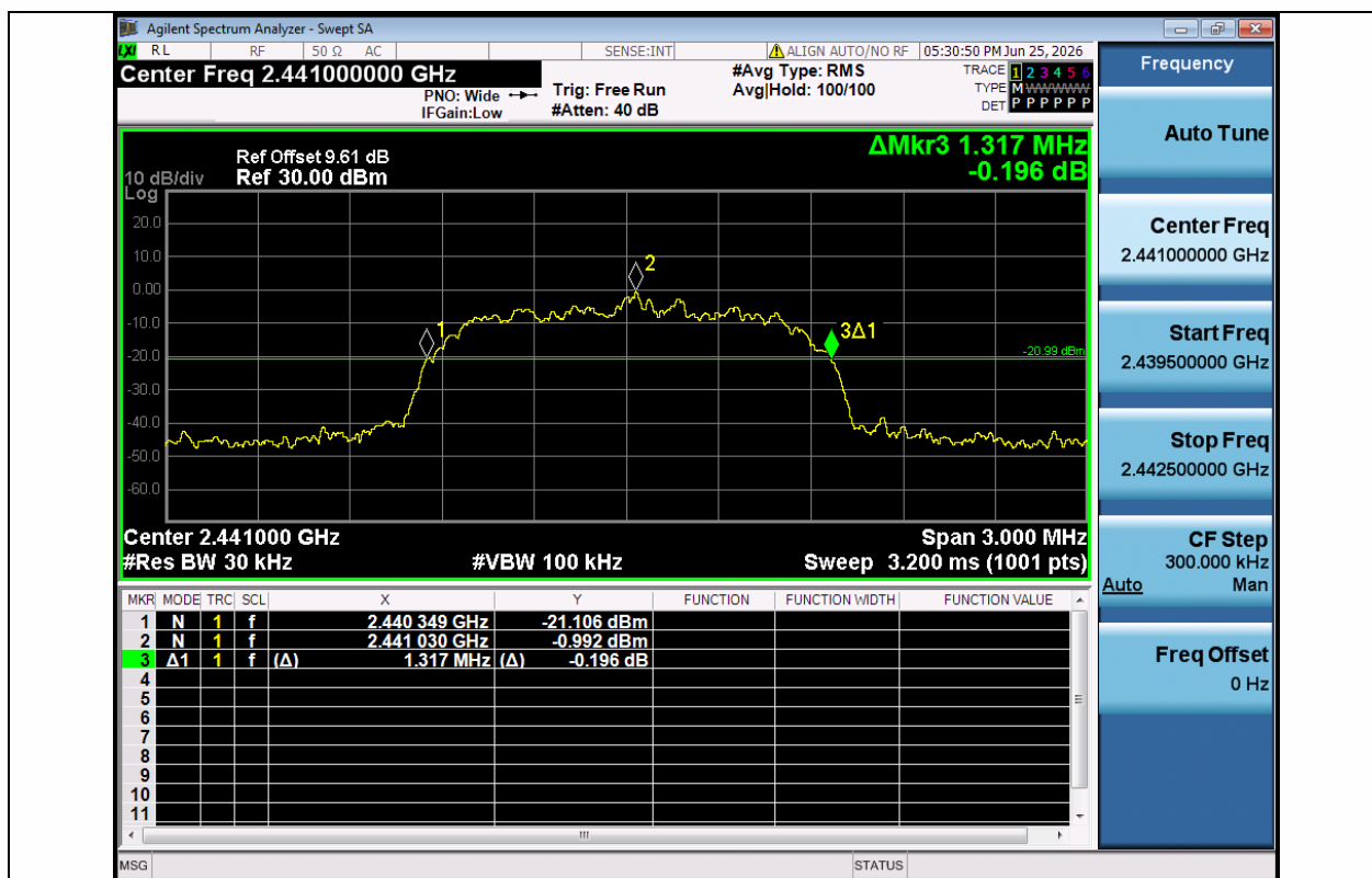
2DH5-Ant1-2441
