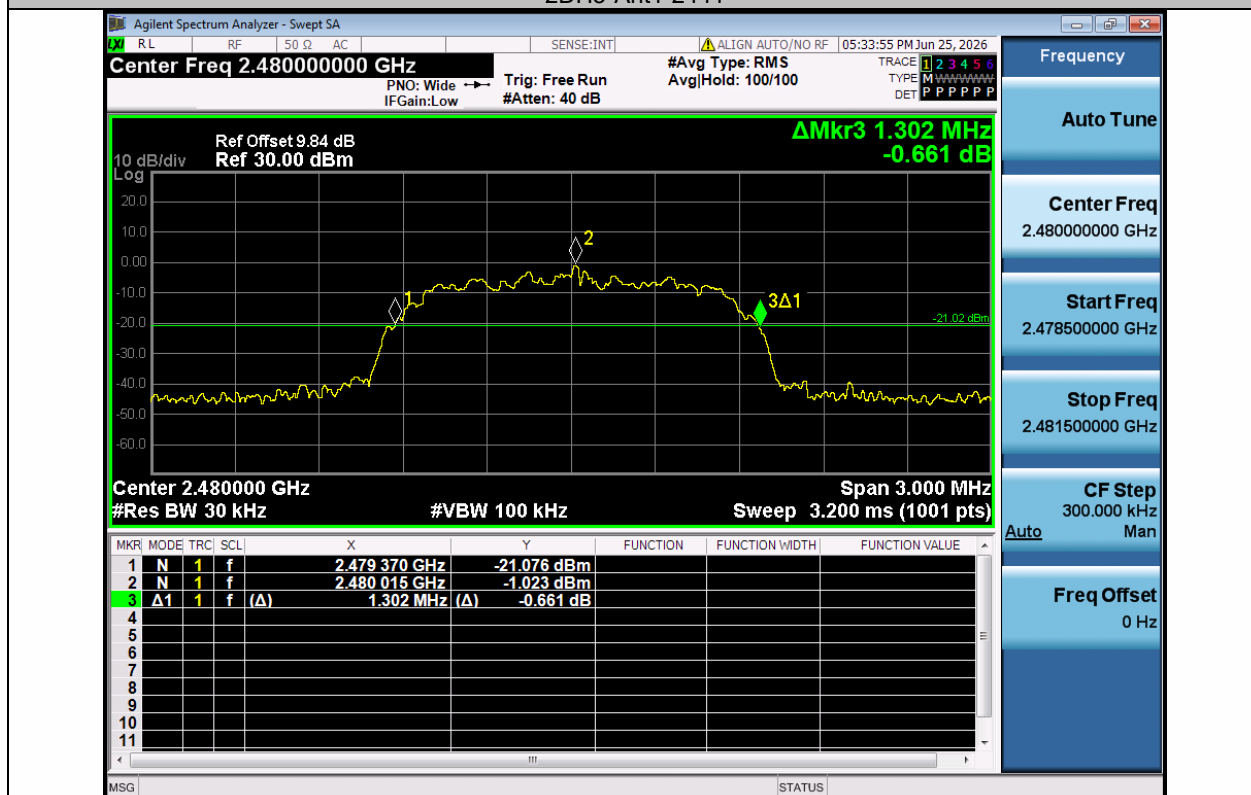
2DH5-Ant1-2480
