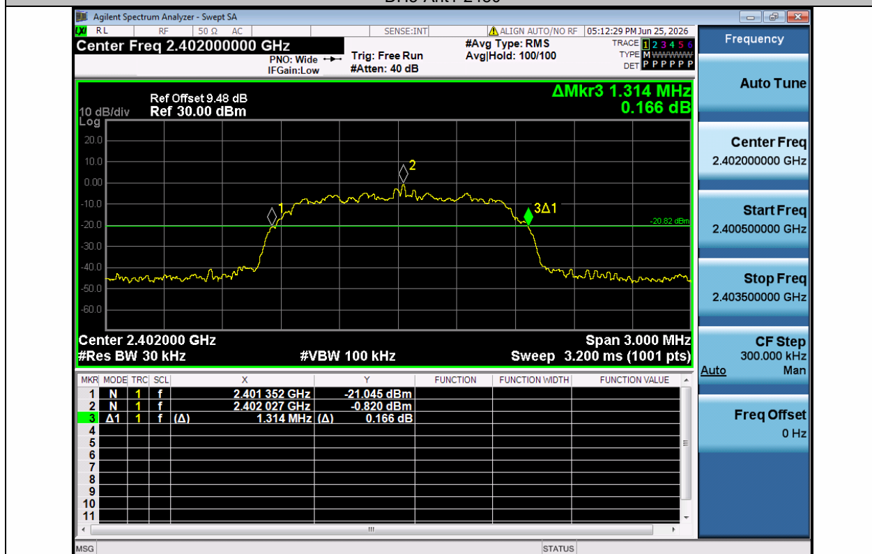
2DH5-Ant1-2402
