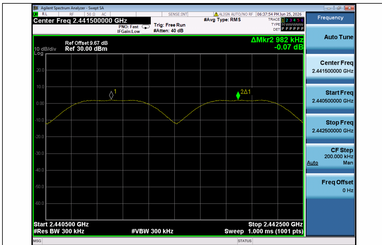
DH5-Ant1-Hop-PASS
