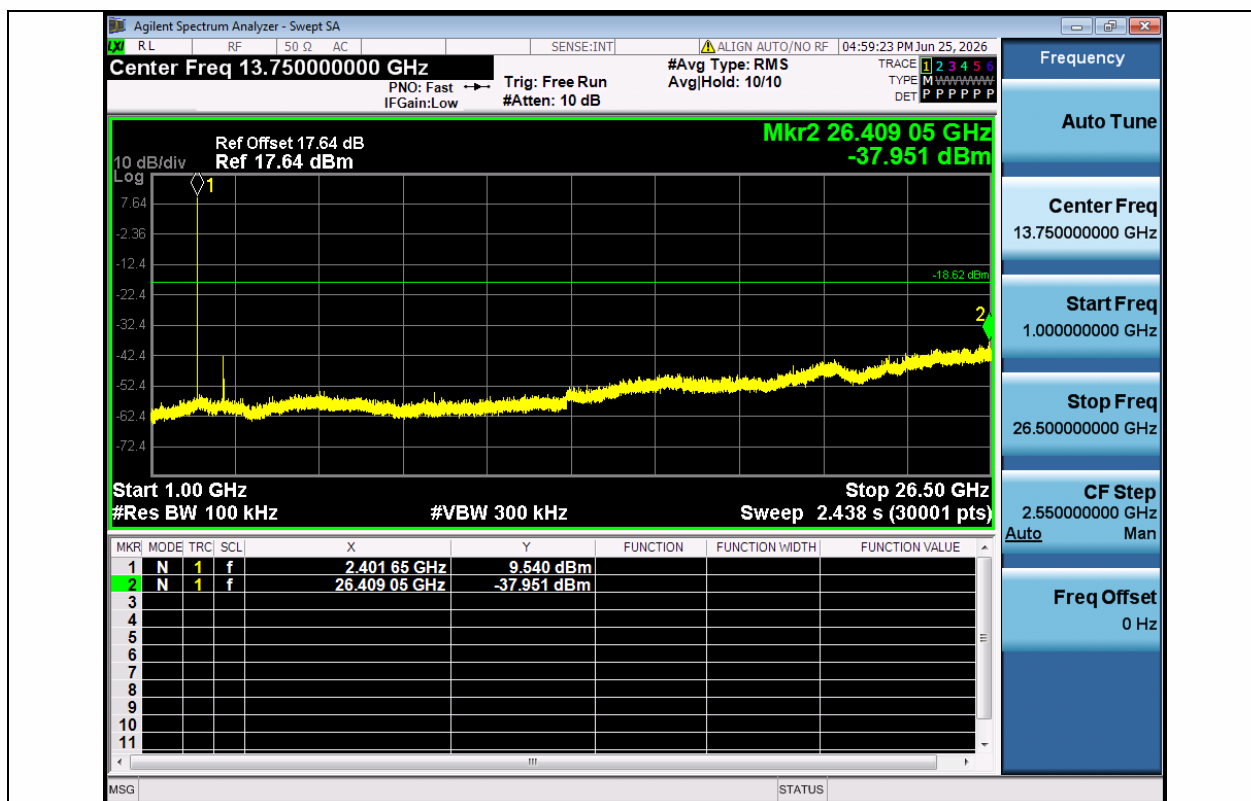
DH5-Ant1-2402-1000~26500-PASS
