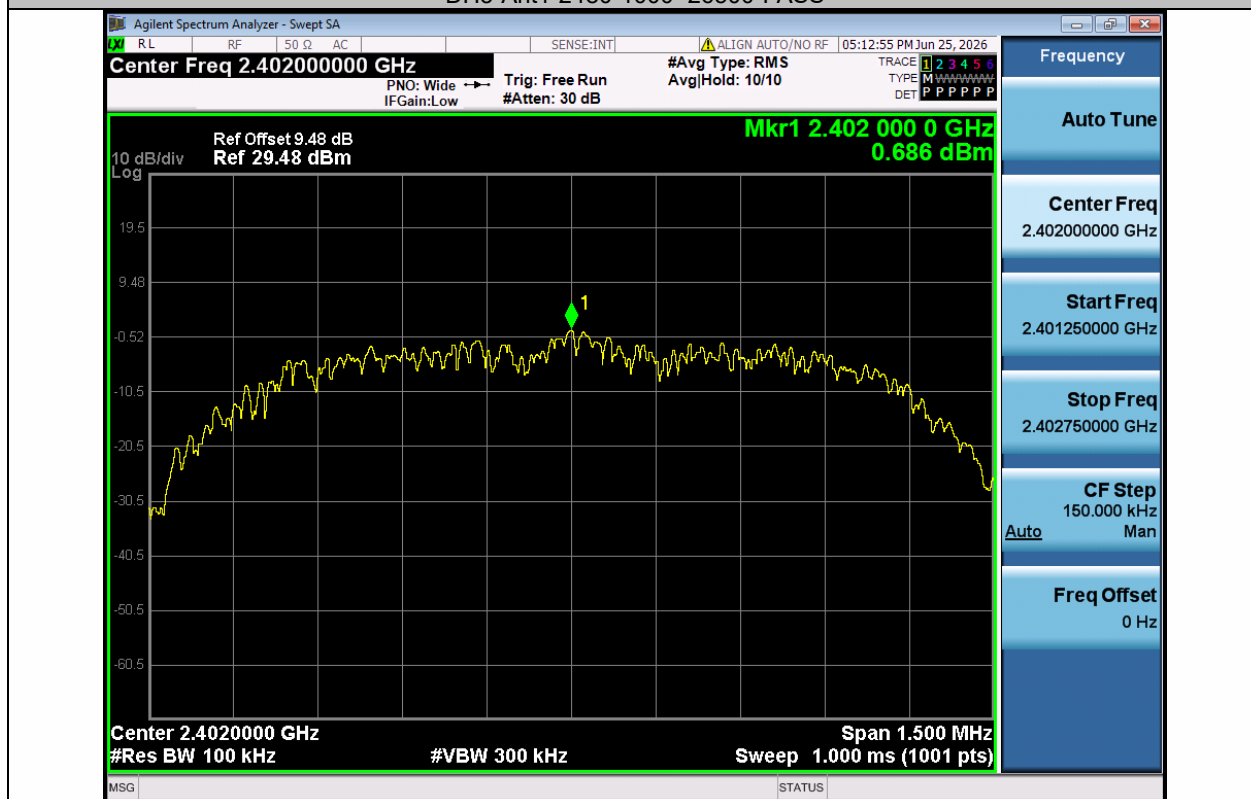
2DH5-Ant1-2402-0~Reference-PASS
