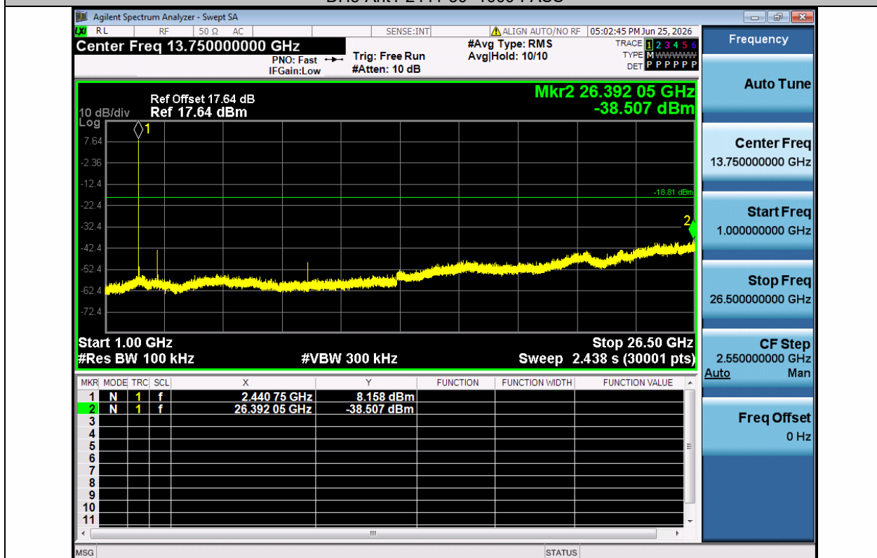
DH5-Ant1-2441-1000~26500-PASS
