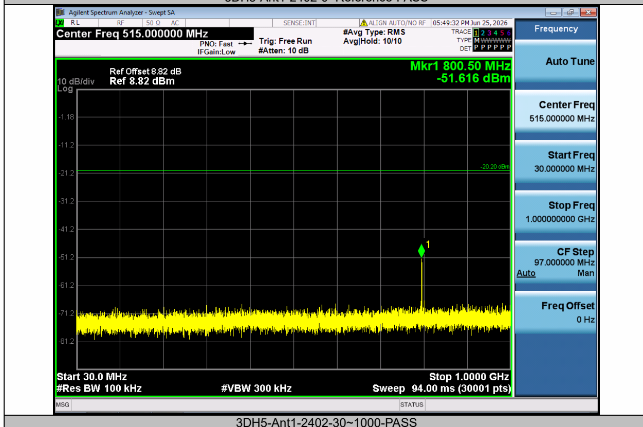
3DH5-Ant1-2402-30~1000-PASS
