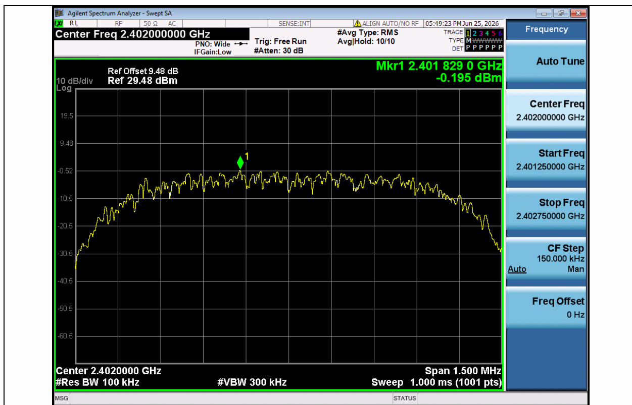
3DH5-Ant1-2402-0~Reference-PASS
