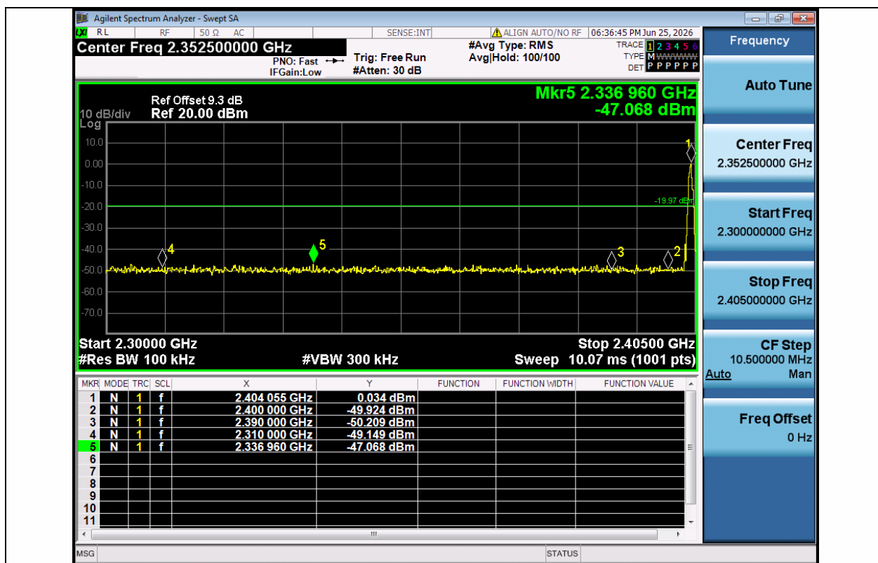
DH5-Ant1-Hop_2402-PASS
