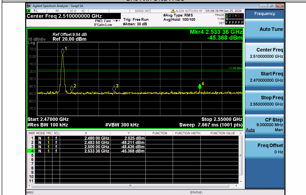
DH5-Ant1-2480-PASS
