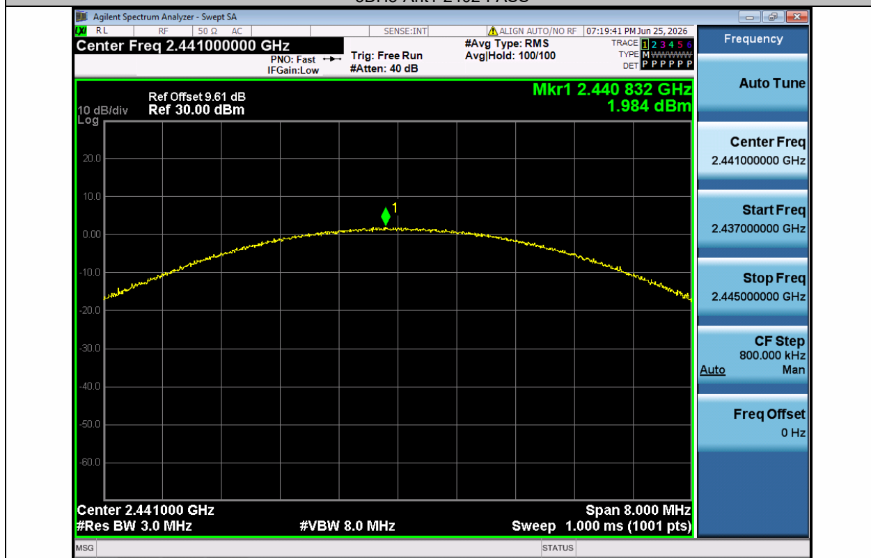
3DH5-Ant1-2441-PASS
