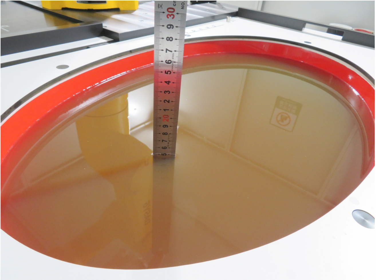
15cm Depth Head Tissue for SAM Phantom
