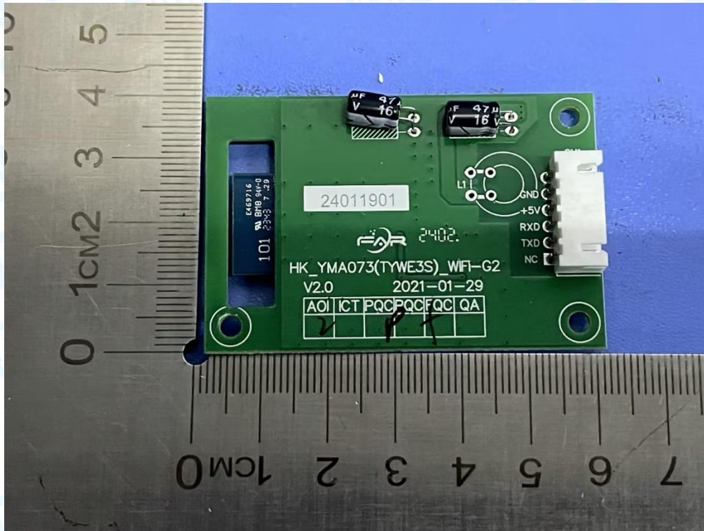
Photo 13 Appearance of PCB
