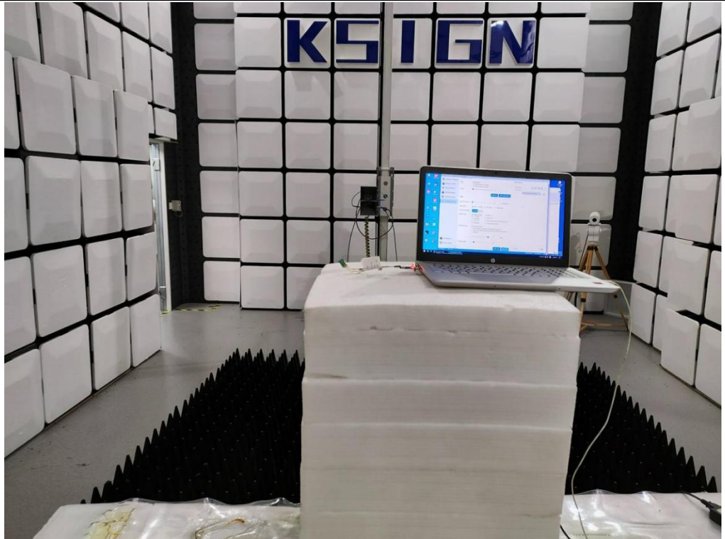
Emissions in restricted frequency bands (above 1GHz) / MK16A
